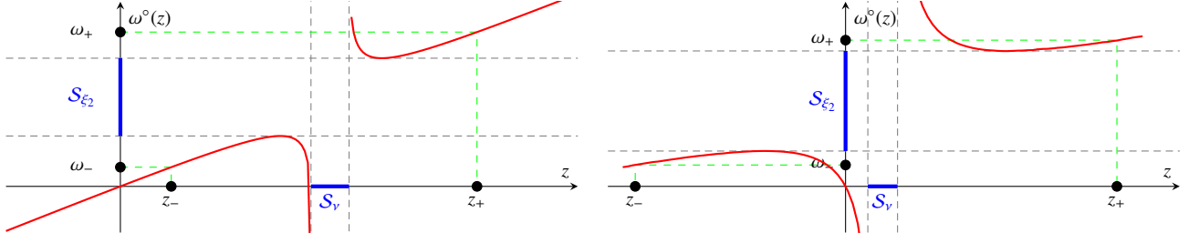
Fig. C.9: Variable change z \mapsto \omega^\circ(z) = z + c_2^\infty \int \frac{zdv(t)}{z-t} for c_2^\infty < 1 (left) and c_2^\infty > 1 (right). S_\theta is the support of the probability measure \theta . For 0 < \omega_- = \omega(z_-) < \inf S_\gamma , the pre-image z_- is necessarily negative for c_2^\infty > 1 .
