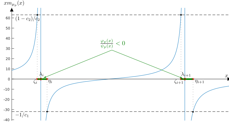
Fig. B.4: Visual representation of x \mapsto M_p(x) = xm_{\mu_p}(x) ; here for p = 4, n_1 = 8, n_2 = 16 . Solutions to M_p(x) = -1/c_1 (i.e., \eta_i 's) and to M_p(x) = (1 - c_2)/c_2 (i.e., \zeta_i 's) indicated in red crosses. Green solid lines indicate sets of negative \varphi_p/\psi_p .
