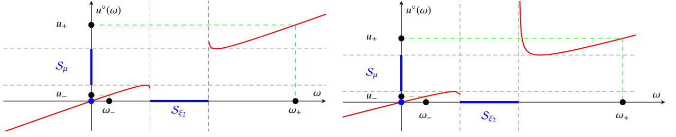
Fig. C.10: Variable change u^o(\omega) = (\frac{1}{\omega} + c_1^\infty \int \frac{1}{t-\omega} d\xi_2(t))^{-1} for c_2^\infty < 1 (left) and c_2^\infty > 1 (right). S_\theta is the support of the probability measure \theta .
