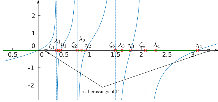
Fig. B.6: Example of visual representation of \varphi_p/\psi_p : \mathbb{R} \rightarrow \mathbb{R} , x \mapsto \varphi_p(x)/\psi_p(x) ; here for p = 4 , n_1 = 8 , n_2 = 16 . In green solid lines are stressed the sets over which \varphi_p(x)/\psi_p(x) < 0 (which correspond to branch cuts in the study of f(z) = \ln^k(z) ). Possible real crossings of the contour \Gamma are indicated, notably showing that no branch cut is passed through when f(z) = \ln^k(z) .
