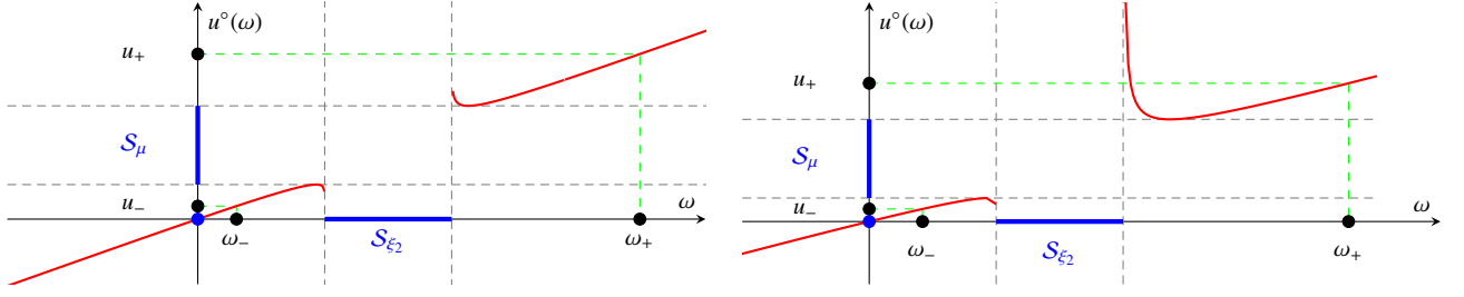
Fig. C.10: Variable change u^\circ(\omega) = (\frac{1}{\omega} + c_1^\infty \int \frac{1}{t-\omega} d\xi_2(t))^{-1} for c_2^\infty < 1 (left) and c_2^\infty > 1 (right). S_\theta is the support of the probability measure \theta .
