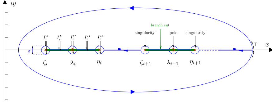
Fig. B.7: Chosen integration contour. The set I_i^B is the disjoint union of the segments [\zeta_i + \varepsilon + 0^+ \iota, \lambda_i - \varepsilon + 0^+ \iota] and [\zeta_i + \varepsilon + 0^- \iota, \lambda_i - \varepsilon + 0^- \iota] . Similarly the set I_i^D is the disjoint union of the segments [\lambda_i + \varepsilon + 0^+ \iota, \eta_i - \varepsilon + 0^+ \iota] and [\lambda_i + \varepsilon + 0^- \iota, \eta_i - \varepsilon + 0^- \iota] . The sets I_i^A , I_i^C and I_i^E are the disjoint unions of semi-circles (in the upper- or lower-half complex plane) of diameters \varepsilon surrounding \zeta_i , \lambda_i and \eta_i respectively.
