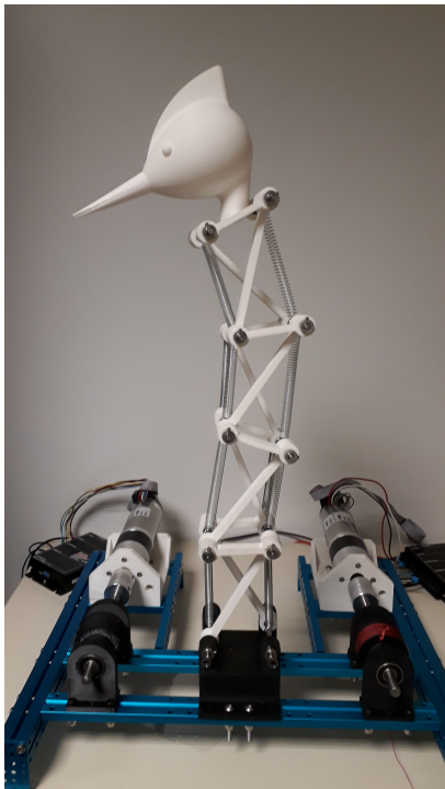
Fig. 6: The prototype under construction.
