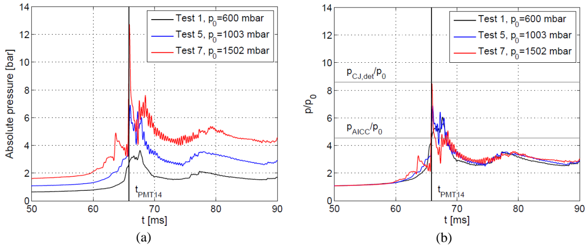
Figure 9. Influence of the initial pressure p_0 on the pressure peaks recorded by PP9: (a) absolute pressure; (b) absolute pressure to initial pressure ratio.
