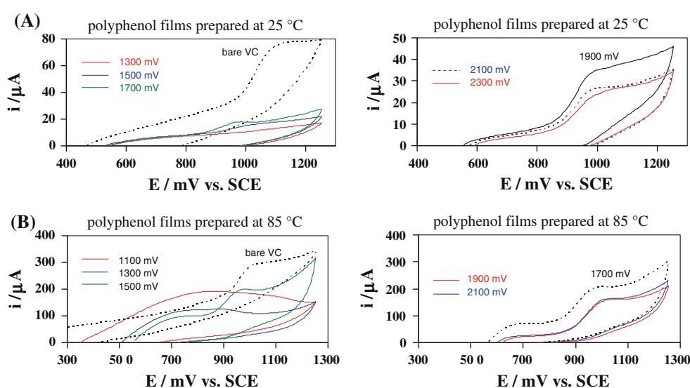
Fig. 10 Cyclic voltammograms (first cycles) recorded on bare and polyphenol film-coated vitreous carbon electrodes in 1 mol L -1 H 2 SO 4 aqueous solution containing 1 mmol L -1 phenol at 25 °C (a) and 85 °C (b). Scan rate: 100 mV s -1 . The polyphenol films were prepared by anodic polarization at various applied potentials (1,100–2,300 mV) for 10 min in 1 mol L -1 H 2 SO 4 aqueous solution containing 1 mmol L -1 phenol at 25 °C (a) and 85 °C (b)
