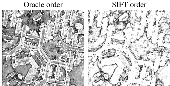
Figure 5: Reconstruction error of the DSM obtained with bundle adjustment of camera rotations (IARPA AOI), using the oracle and the SIFT orders. Brighter values account for larger errors. Errors above 1 m are clipped and correspond to white pixels.
