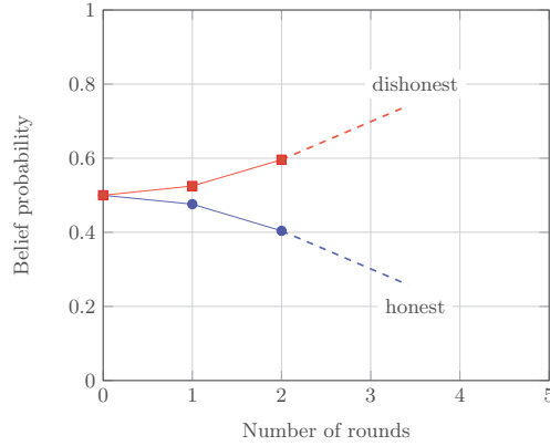
Fig. 6: The progressive change in the beliefs of the Jury type \mathbf{tj}_U about the type of S
