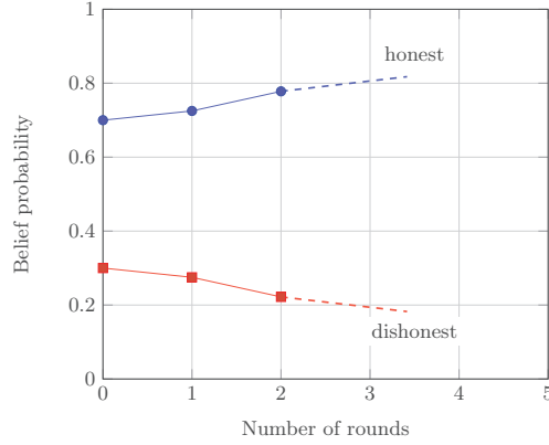
Fig. 7: The progressive change in the beliefs of the Jury type \mathbf{tj}_B about the type of S
