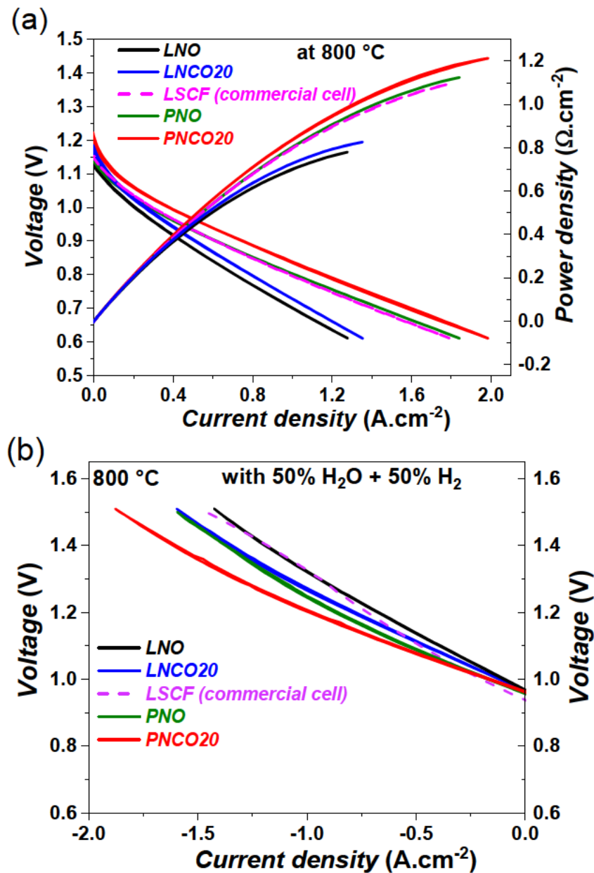
Figure 5. Current density-voltage relationship curves, at 800 \text{ }^\circ\text{C} for single cell containing \text{Ln}_2\text{Ni}_{1-x}\text{Co}_x\text{O}_{4+\delta} ( \text{Ln} = \text{La}, \text{Pr} and x = 0.0 and 0.2 ) and compared with commercial LSCF cell; (a) under SOFC mode and (b) under SOEC mode with 50\% \text{ H}_2 + 50\% \text{ H}_2\text{O} feed gas mixture.
