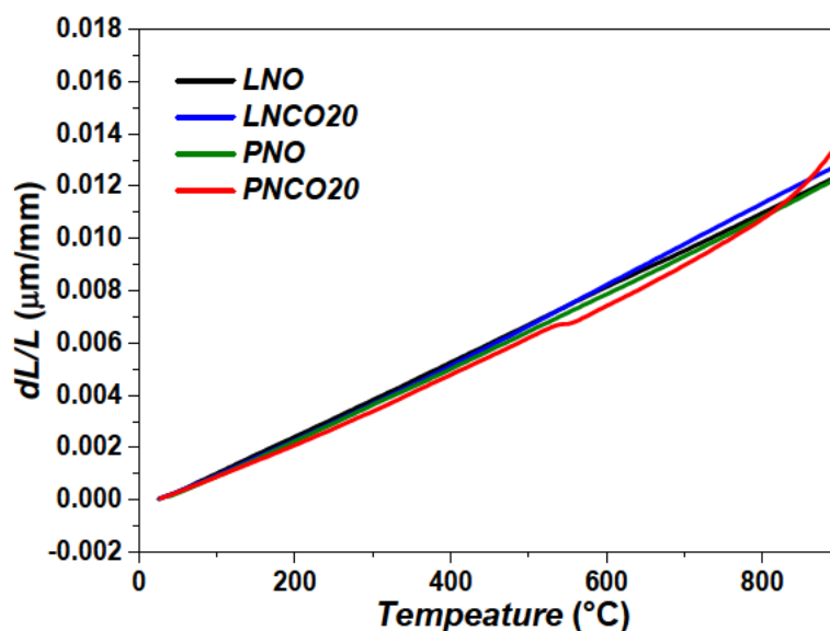
Figure 3. Thermal variation and relative expansion ( dL/L ) for \text{Ln}_2\text{Ni}_{1-x}\text{Co}_x\text{O}_{4+\delta} ( \text{Ln} = \text{La}, \text{Pr} and x = 0.0 and 0.2 ), under air ( 30 \leq T \leq 900^\circ\text{C} ).
