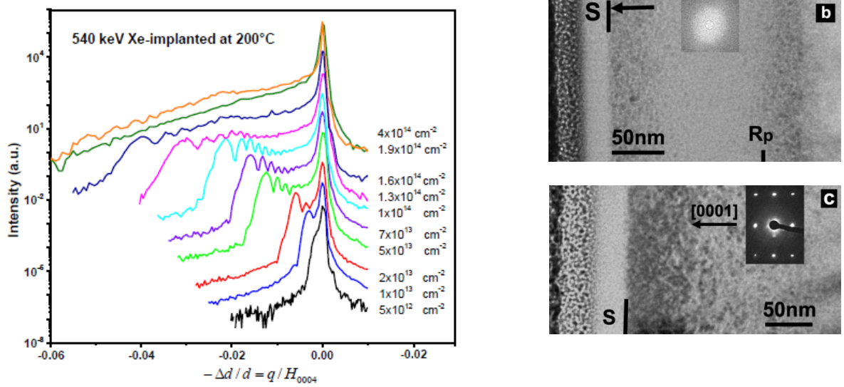
Figure 1. Left: evolution with increasing fluences of the X-ray scattered intensity distribution along the surface direction close to the (0004) reflection of SiC implanted with 540 keV xenon ions at 200°C ( \Delta d/d ) is the normal strain- Right: XTEM images of SiC implanted at 1.2 dpa (b) and 0.6 dpa (c)
