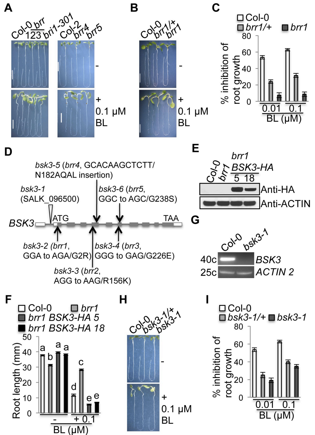
Fig 1. Identification of five semi-dominant mutations in BSK3. (A-C) Root growth of Col-0 and brr mutants (+/- BL). (D) The gene structure of BSK3. Arrows point to the positions of five identified BSK3 mutations. White boxes represent 5' UTR and 3' UTR. Gray boxes and lines represent exons and introns, respectively. Triangle represents the T-DNA insert, and the insertion is in the first intron in the 5' UTR of BSK3. (E) Western blot analysis of BSK3-HA protein expression in two brr1 BSK3-HA lines. Thirty micrograms of total proteins were loaded. (F) Primary root length of Col-0, brr1 , and brr1 BSK3-HA seedlings. Different letters above the bars indicate significant differences ( P < 0.05 ). (G) RT-PCR analysis of BSK3 gene expression. ACTIN2-FW/ACTIN2-RV and BSK3-FW/BSK3-RV primers were used to amplify ACTIN2 (25 cycles) and BSK3 (40 cycles) transcripts, respectively. (H and I) Root growth of Col-0, bsk3-1/+ , and bsk3-1 seedlings (+/- BL). (A-C and E-I) Seedlings were grown in the light for 7 days. Error bars represent SEM ( n = 36-60 ). Scale bar = 0.5 cm.
