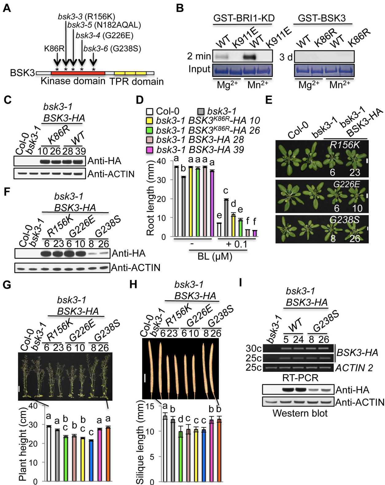
Fig 3. Kinase dead BSK3 K86R protein partially rescues the bsk3-1 mutant phenotypes. (A) BSK3 mutations in the kinase domain. The kinase domain (58–312 aa) of BSK3 was predicted by SMART (Simple Modular Architecture Research Tool, http://smart.embl-heidelberg.de/ ). (B) In vitro kinase assays. About 10–20 μg of GST fusion proteins were loaded for kinase assays. Dried protein gels were exposed to films for 2 minutes (GST-BRI1-KD and GST-BRI1-KD K911E ) or 3 days (GST-BSK3 and GST-BSK3 K86R ) at –80 °C. (C) Western blot analyses of BSK3-HA and
