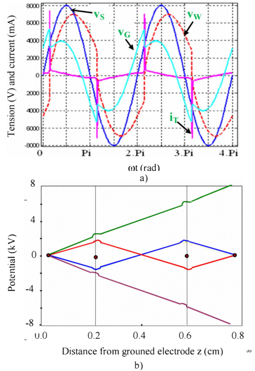
Figure 2: (a) Temporal variations of the source voltage v_s(t) , voltage in the gap v_G(t) , voltage between the barriers v_w(t) and total current i_T(t) under sine voltage waveform with f = 50\text{kHz} , total pressure = 400Torr, rate of mixture Xe/Cl 2 = 97:03, V_s = 8\text{kV} ; (b) Potential distributions between the electrodes for \omega t = 0,5\pi, \pi, 1,5\pi and 2\pi . Here the vertical lines at z=0.2\text{cm} and 0.6\text{cm} represent the barrier surfaces.
