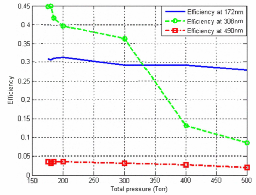
Figure 4: Influence of the total pressure on the efficiency of the XeCl excilamp supplied with a sine waveform source at V=8\text{kV} , f=50\text{kHz} and composition of Xe:Cl 2 =97:3(%)
