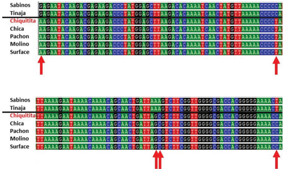
Figure 6. Fragment of the mitochondrial 16S rRNA. Individuals from Chiquitita Cave have identical sequence to members of the “A” lineage (Chica cave, Pachón cave, Molino cave and Rio Comandante surface river). Members of the “B” lineage (Sabinos cave and Tinaja cave) have 5-6 bp disagreements in this fragment, indicated by red arrows.
