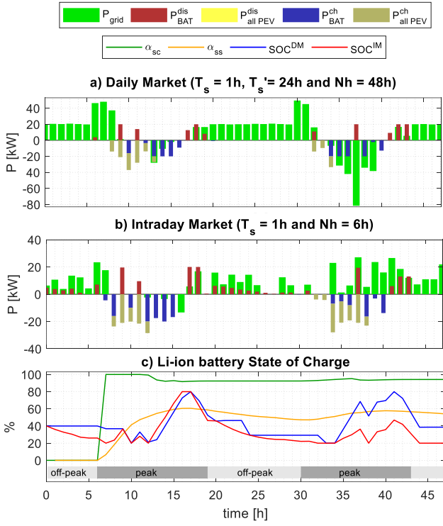
Fig. 5: H MPC with disturbances. (a) MPC1 variables in DM time frame. (b) MPC2 variables in IM time frame. (c) Li-ion batteries SoC, self-consumption and self-sufficiency index in the two days.
