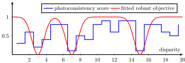
Figure 3: The conversion of photo-consistency scores into a robust objective with multiple local minima.
