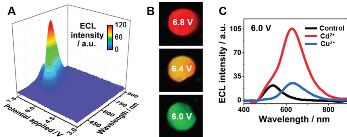
Figure 4. Potential-resolved BPE-induced ECL spectrum recorded with a mixture of Ir(ppy) 3 and Ru(bpy) 3 2+ dyes (A). Series of potential-dependent images of the anodic pole of the closed bipolar electrode (B). Characteristic ECL spectra in the absence or presence of metal cations (C). Adapted from ref. [50]. Copyright © (2019) Royal Society of Chemistry
