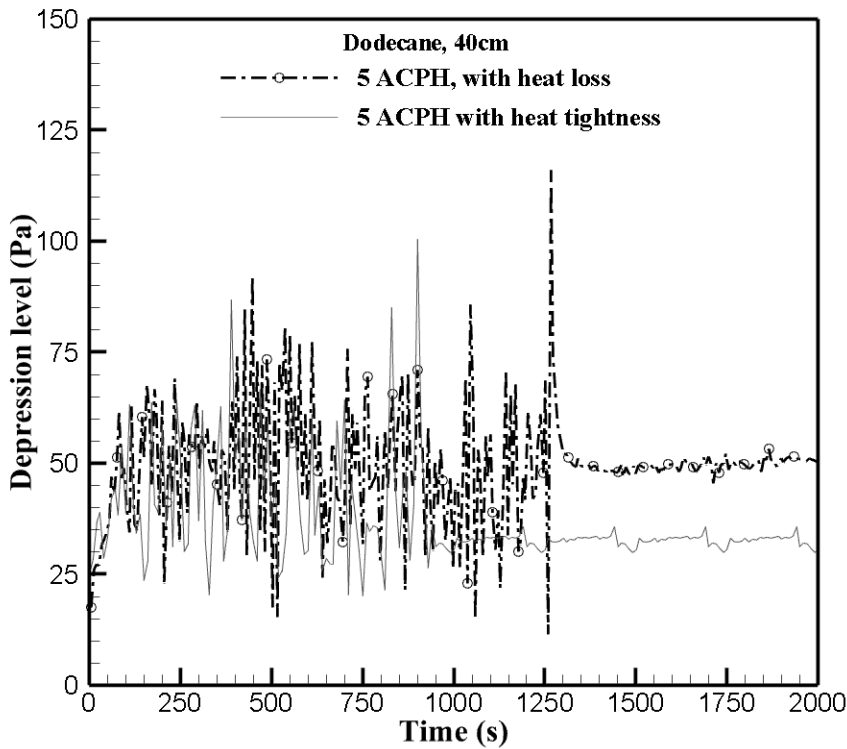
Figure 3. Impact of the intermediate levels of thermal insulation on the pressure inside enclosure
