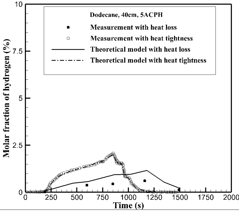
Figure 15. Effect of the intermediate levels of thermal insulation on hydrogen concentration in transient mode at entrance of the extraction duct
