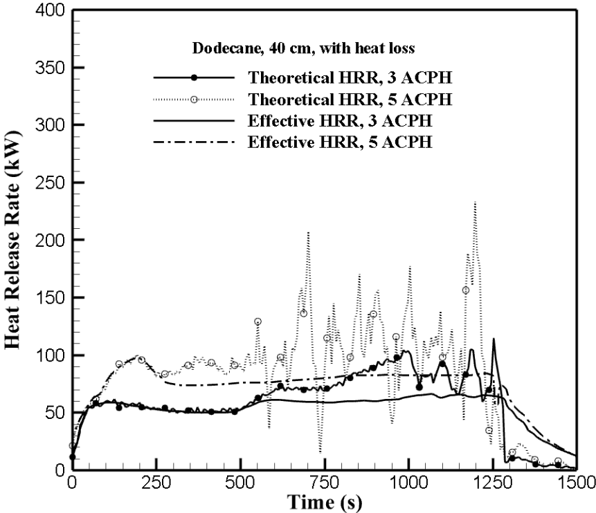
7a) with heat loss
