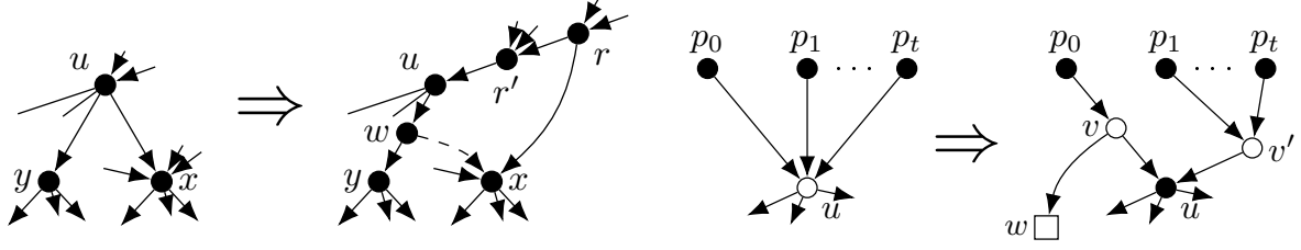
Figure 5: Illustration of Rule 3 (left) and Rule 4 (right). Triangles are leaves and children of the initial vertex \psi , white vertices are children of the root \rho . Note that, on the left, u has a tree-vertex child before and after the modification.
