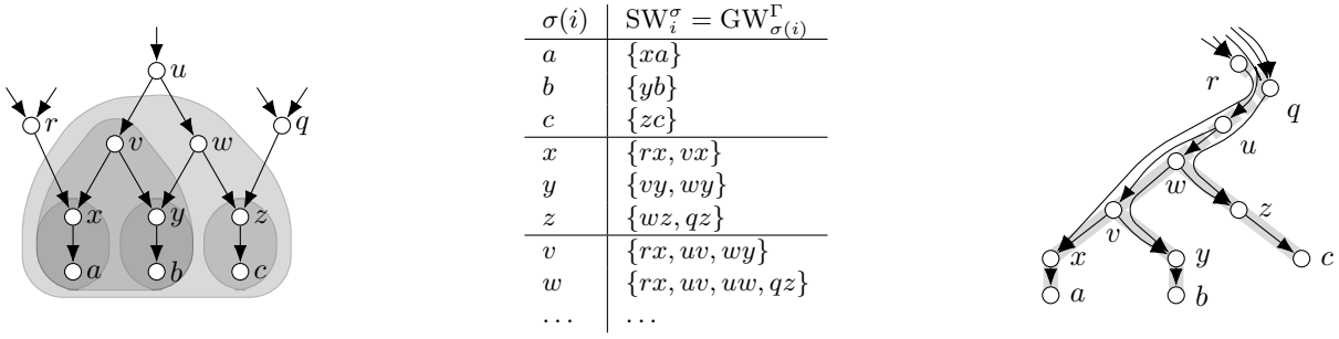
Figure 3: Illustration of the two definitions of scanwidth. Left: Lower part of a graph G where gray zones represent the weakly connected components induced by \sigma[1..i] for \sigma = (a, b, c, x, y, z, v, w, \dots) and i \leq 8 . Here, \text{SW}_v^\sigma = \{rx, uv, wy\} since x, y, and v are weakly connected in G[a, b, c, x, y, z, v] . Middle: table indicating \text{SW}_i^\sigma for i \leq 8 corresponding to \sigma . Right: part of a tree \Gamma with \text{GW}_{\sigma(i)}^\Gamma = \text{SW}_i^\sigma for all i \leq 8 . For the extension \pi = (c, a, z, b, y, x, v, w, \dots) , we also have \text{GW}_{\pi(i)}^\Gamma = \text{SW}_i^\pi for all i \leq 8 .
