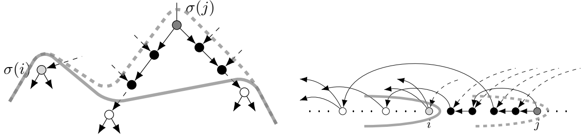
Figure 2: Left: For an extension \sigma each position i induces a cut through G separating the vertices in \sigma[1..i] (below gray line) from \sigma[i+1..] (above gray line). Right: G with vertices linearly arranged according to \sigma .
