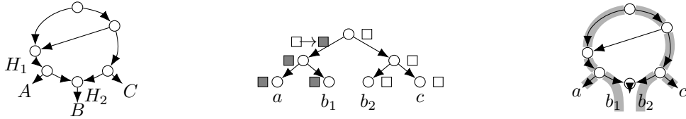
Figure 1: Left: A phylogenetic network N depicting the evolutionary history of species A , B , and C . Center: An evolution scenario for a gene, given the sequences of one individual from species A , one from C and two from B , where different alleles (boxes) are observed: gray for A and for one individual from B , and white for the other individuals. The arc containing the mutation from the white to the gray allele is marked. Right: An embedding (gray arcs) in N of this gene evolution scenario.
