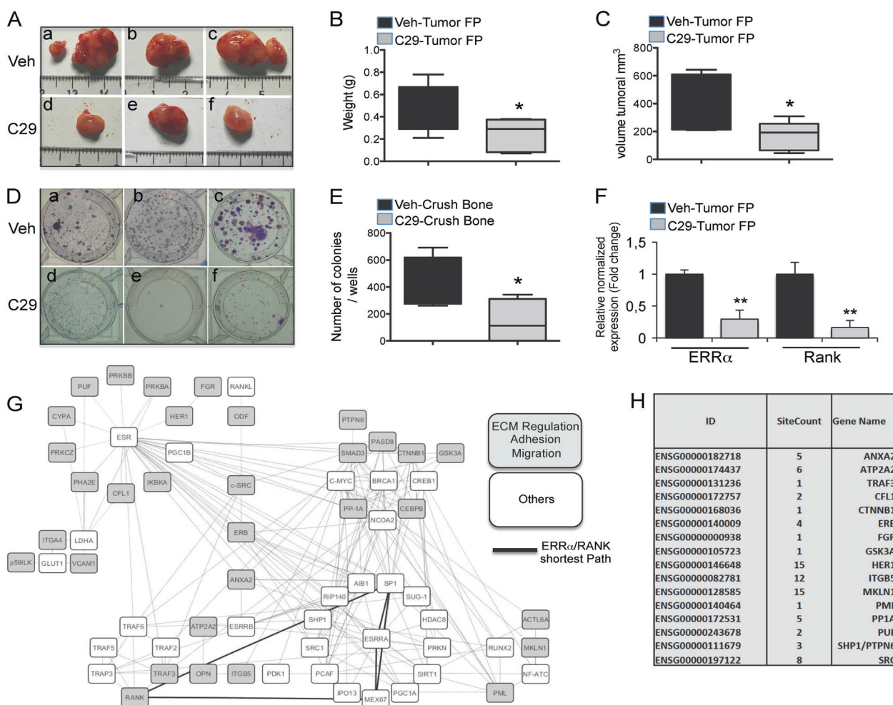
Fig. 5 Pharmacological inhibition of ERR\alpha . A 4T1- ERR\alpha (clones 1–3) cells were inoculated into the FP of the mammary gland of BALB/c mice and mice were treated with C29 (10 mg/kg) for 10 days from the time of tumor appearance to tumor resection (day 14). C29 (C29-Tumor-FP) ( d–f ) decreased tumor expansion compared to tumor growth in vehicle treated mice ( a–c ). B , C Weight and volume of tumors dissected at endpoint ( n = 9 , unpaired t -test, weight: P = 0.014 ; Mann and Whitney; volume: P = 0.019 ). D , E After tumor resection, animals were kept for an additional 21 days, bones were then crushed and released cells were cultured for 3 weeks. C29 treatment ( d–f ; E ) decreased TCB number compared Veh ( Da–c ; E ) ( n = 5 , 142 \pm 138 versus 416 \pm 138 , unpaired t -test, P = 0.035 ). F Real-time PCR
