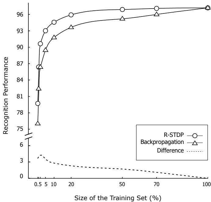
Figure 3: Comparison of recognition performances of the proposed network and a supervised SNN [20] while training them with restricted training set.
