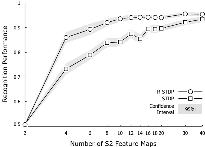
Figure 5: Comparison of recognition performance when STDP or R-STDP is applied to S_2 in Task 2. Superiority of R-STDP over STDP in finding diagnostic features (and discarding distractors) is clearly shown when there are small number of feature maps in S_2 . As the number of feature maps increases, STDP has more chance to extract features for target digits, therefore approaches the performance of applying R-STDP. With respect to the number of feature maps, R-STDP shows a monotonic behavior in increasing the performance and confidence level, however, STDP is not as robust as R-STDP, specially in terms of confidence level.
