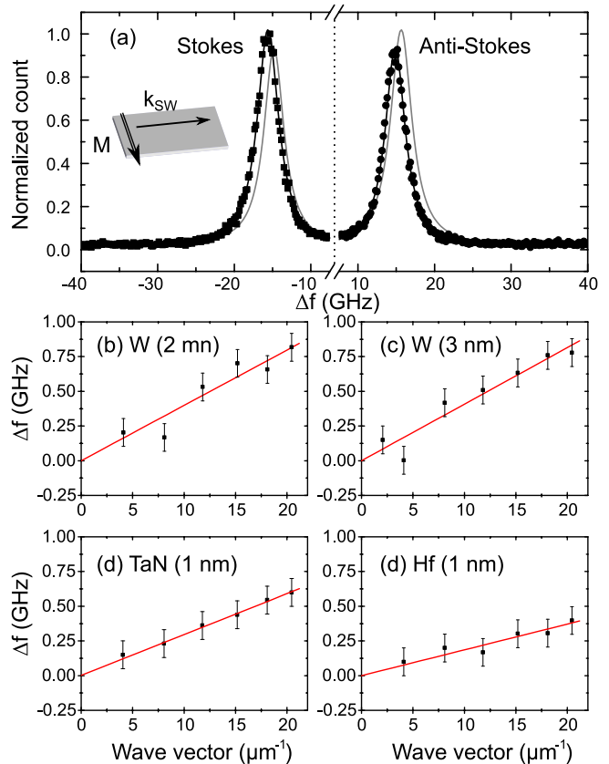
FIG. 4. (a) BLS spectra measured for the 2 nm thick W underlayer at a light incidence corresponding to k_{\text{sw}} = 20.45 \mu\text{m}^{-1} and an in-plane field of 1T to saturate the magnetization. Lorentzian fit are also superposed to show the nonreciprocal behavior of the spin-wave, in gray the Stokes and anti-Stokes are inverted. The inset shows a schematic illustration of the Damon-Eshbach configuration used. (b)-(e) Linear fit of the frequency difference \Delta f as a function of wave vector for the different underlayers.
