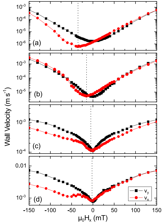
FIG. 3. (Color online) Domain wall velocity as a function of in-plane applied field H_x for propagation along (squares) and perpendicular (circles) to the field direction. The propagation takes place under a static perpendicular field, H_z . (a) 2 nm thick W underlayer at \mu_0 H_z = 2.8 mT. (b) 3 nm thick W underlayer at \mu_0 H_z = 2.9 mT. (c) 1 nm thick TaN underlayer at \mu_0 H_z = 0.83 mT. (d) 1 nm thick Hf underlayer at \mu_0 H_z = 2.9 mT. The dashed vertical line indicates the offset field, H_{\text{offset}} .
