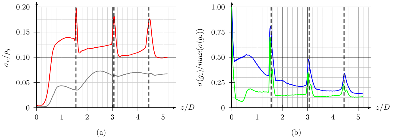
Figure 10. Axial evolution of (a) density fluctuations, taken along \text{---} r/D=0.63 and \text{---} \text{---} the line of maximum density fluctuations, (b) the maximum of gray levels g_i fluctuations, considering either schlieren images obtained with a knife-edge oriented along the jet axis ( g_y , \text{---} ) or normal to the jet axis ( g_z , \text{---} ). The dashed vertical lines correspond to the shock positions.
