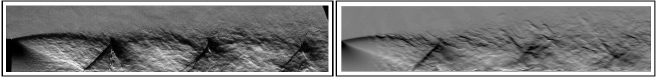
Figure 6. Schlieren images obtained from experiments 7 at Re_D = 2 \times 10^6 (left) and from the simulation at Re_D = 5 \times 10^4 (right).
