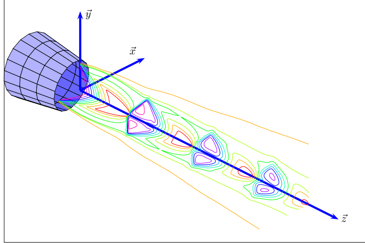
Figure 2. Time-averaged density field of an underexpanded, M_j = 1.56 and Re_D = 5 \times 10^4 , jet, obtained by simulation. 16 Isovalues of density from 1 to 2.6 \text{kg}\cdot\text{m}^{-3} , by step 0.2 \text{kg}\cdot\text{m}^{-3} , are presented.
