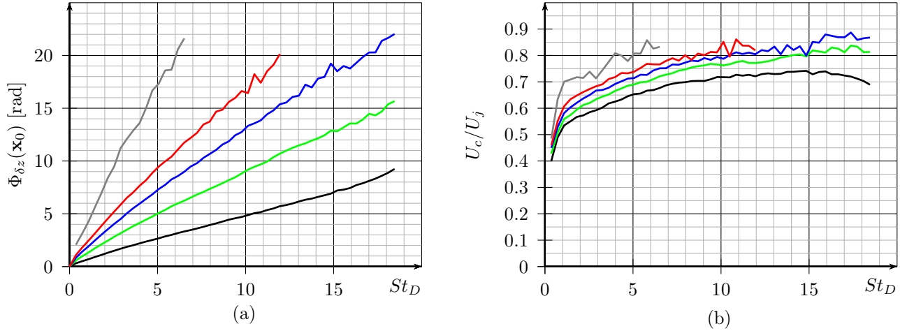
Figure 3. (a) Phase lag \Phi_{\delta z}(\mathbf{x}_0) for different couples of points centered on x_0 : \blacksquare \delta_z = 4 px; \blacksquare \delta_z = 8 px; \blacksquare \delta_z = 12 px; \blacksquare \delta_z = 16 px; \blacksquare \delta_z = 32 px, (b) Estimation of the non-dimensioned convection velocity U_c/U_j for the same couples of points centered on x_0
