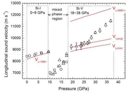
Figure 1. Longitudinal sound velocities of silicon as a function of pressure.
