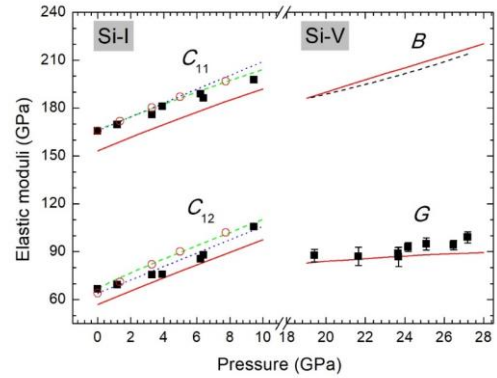
Figure 2. Pressure dependences of elastic moduli of the Si-I and Si-V phases.
