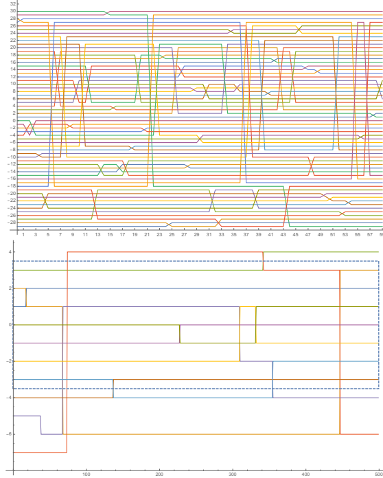
FIGURE 0.1. Left: a simulation of the 60 trajectories (X_i^{(60)})_{-29 \leq i \leq 30} of a uniform minimal factorization of the 60-cycle. Right: a simulation of all the trajectories (X_i^{(500)})_{i \in \mathcal{I}_3^{(500)}} which cross the dashed rectangle [0, 500] \times [-3, 3] ; here \mathcal{I}_3^{(500)} = \{-7, -5, -4, -3, -2, -1, 0, 1, 2, 3\} .
