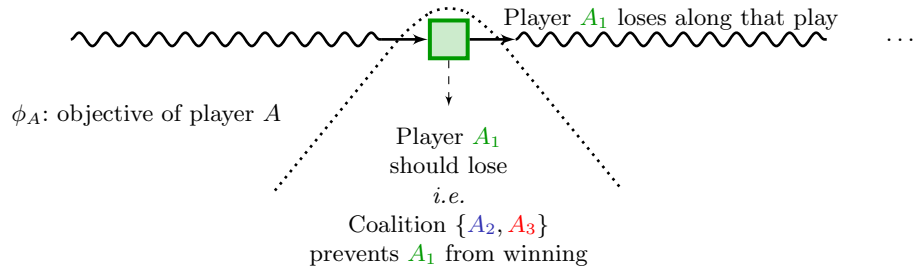
Fig. 3. General shape of a Nash equilibrium in the simple setting (example with three players).
