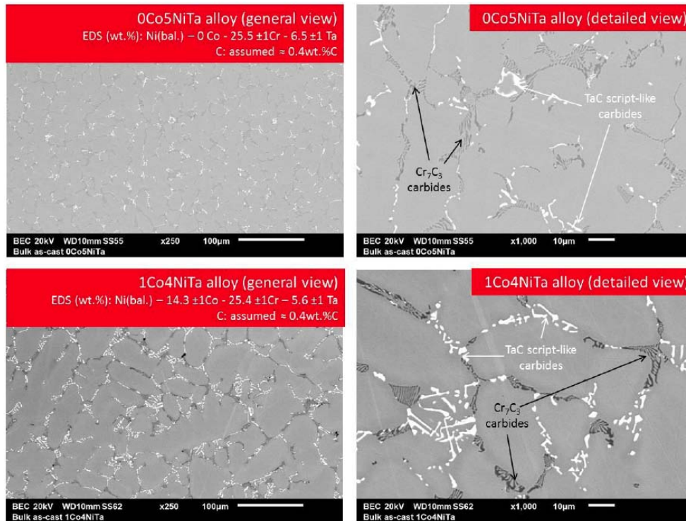
Figure 2: Microstructures of the two nickel-richer alloys in their as-cast states (top: 0Co5NiTa, bottom: 1Co4NiTa, left: ×250, right: ×1000); left: composition measured by 5 full frame EDS on ×250 areas.
