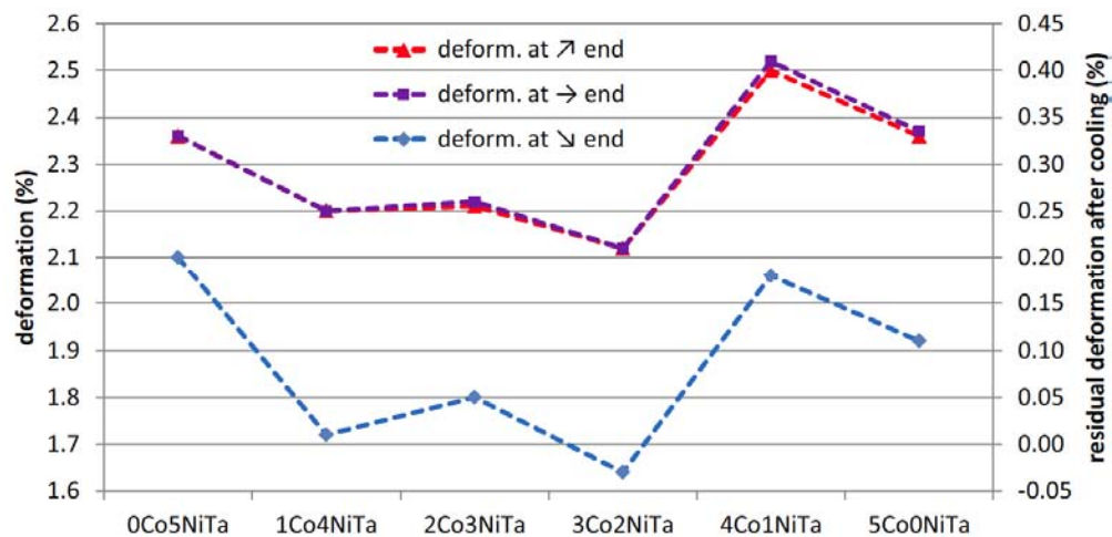
Figure 10: Variation, versus the Co enrichment at the expense of Ni, of the deformation achieved during the whole heating, of the deformation existing at the end of the isothermal stage and the residual deformation after return to room temperature.
