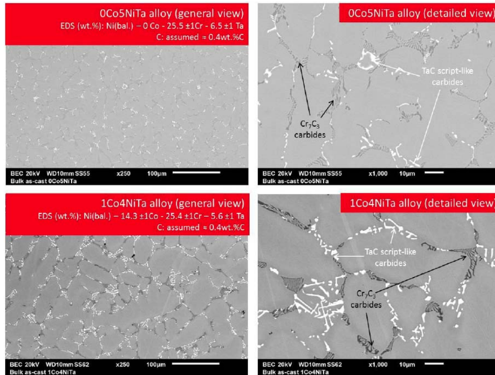
Figure 2: Microstructures of the two nickel-richest alloys in their as-cast states (top: 0Co5NiTa, bottom: 1Co4NiTa, left: \times 250 , right: \times 1000 ); left: composition measured by 5 full frame EDS on \times 250 areas.
