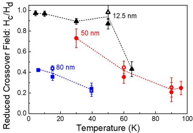
FIG. 4. Temperature variation of the reduced crossover field H_c/H_d for the three sample thicknesses. The filled and empty symbols correspond to the kink of velocity curves (cf. Fig. 1) and the step of \zeta curves (cf. Fig. 3), respectively. The dimensional crossover is shifted toward the depinning transition ( H_c/H_d = 1 ) for decreasing film thickness.
