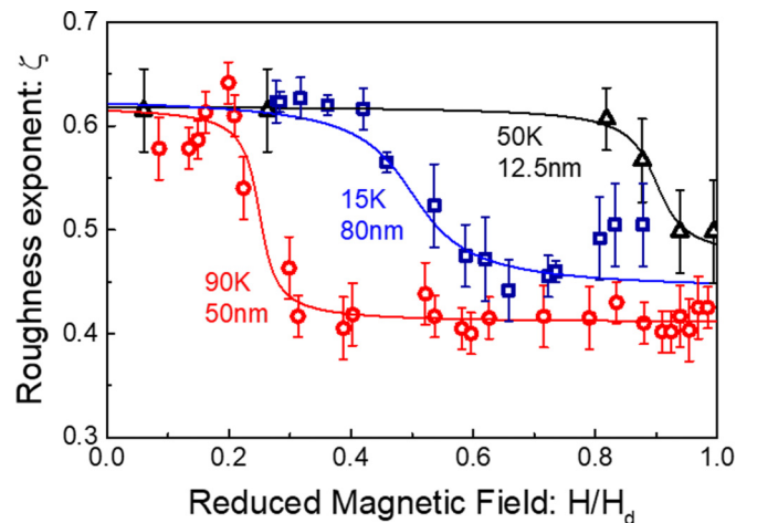
FIG. 3. Roughness exponent \zeta as a function of reduced magnetic field H/H_d for three film thicknesses and different temperatures. The steps between two constant \zeta values reflect a dimensional crossover of DW dynamics. The sigmoidal lines are guides for the eyes. Each error bar corresponds to the standard deviation of average value.
