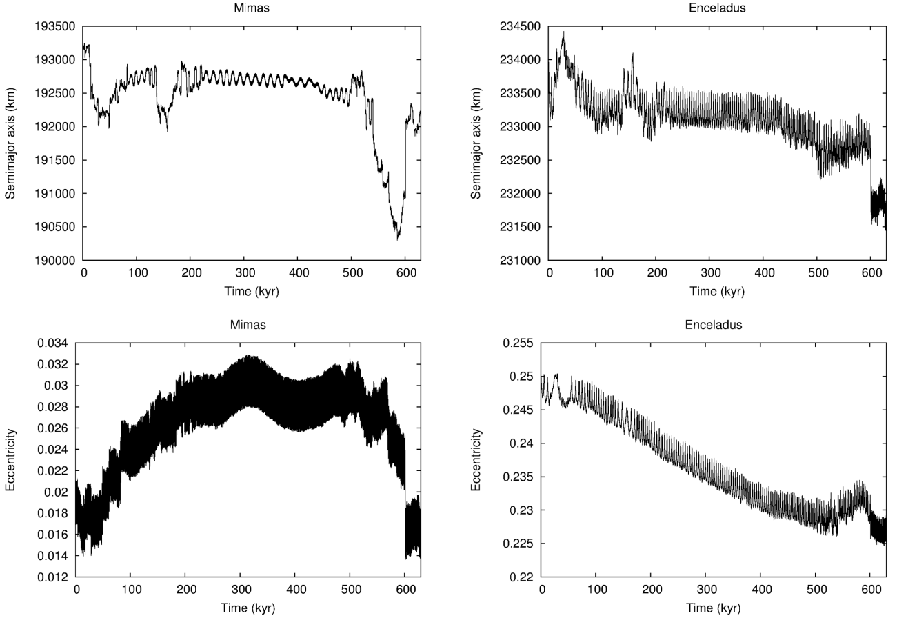
Figure 7. Scenario 2, with Mimas and Enceladus initially close to the 4:3 MMR. Six satellites are present in this simulation. When Enceladus has such a significant eccentricity, the system of the satellites of Saturn is destabilized, which is why all the simulations are stopped before 1 Myr.
