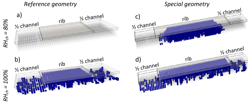
Fig. 9. Liquid water distributions obtained using the MIPNM ( \alpha = 20\% ) for an operating temperature T_{bp} = 80\text{ }^\circ\text{C} and a current density i = 0.75\text{ A}\cdot\text{cm}^{-2} in a cathode GDL unit located under a bipolar plate with L_r = L_{ch} (cases a, b) and a bipolar plate with the rib width twice as large as the channel width ( L_r = 2L_{ch} ) (cases c, d).
