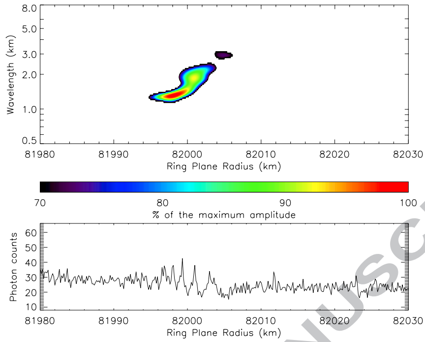
Figure 26. WWZ wavelet power profile of feature 15, computed from co-added wavelet profiles. Lower panel shows the \zeta Orionis, rev. 47 occultation profile.
