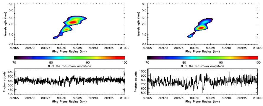
Figure 25. WWZ wavelet power profile of structure 13, computed from individual occultation profiles of \beta Centauri, rev. 77 (left) and \alpha Virginis, rev. 34 (right). Structure 13 is clearly propagating inward on both high incidence and low incidence occultations.
