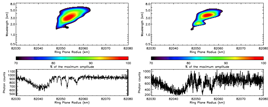
Figure 8. WWZ wavelet power profile of structure 16, computed from co-added wavelet profiles of high-incidence angle occultations (left) and low-incidence angle occultations (right). Lower panels show the \beta Centauri, rev. 85 occultation profile (left) and the \alpha Virginis, rev. 34 occultation profile (right). Structure 16 is located just exterior to the embedded ringlet ER10.
