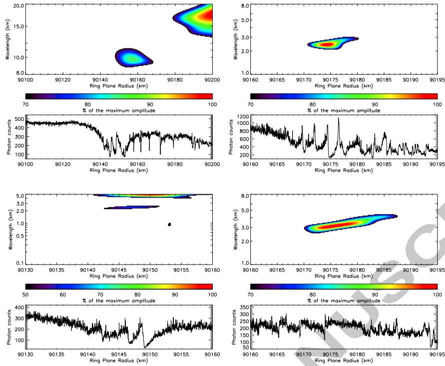
Figure 10. WWZ wavelet power profile of the different parts composing structure 38, computed from individual occultation profile of \beta Centauri, rev. 89 (upper left), \beta Centauri, rev. 64 (upper right), and \beta Centauri, rev. 104 Ingress (bottom). The variety of observed patterns and the local superposition of waves at different wavelengths suggest that this is not a simple bending wave.
