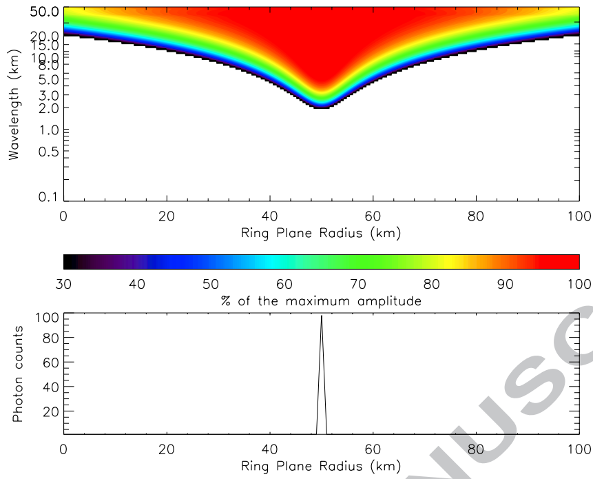
Figure 2. WWZ wavelet power profile for a Dirac signal. The bottom panel presents the simulated data that were analyzed to produce these power transforms.
