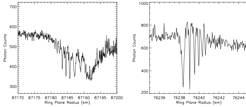
Figure 1. Photon counts from the occultation of \beta Centauri (Rev 75) showing structure 32 propagating inward (left), and of \alpha Virginis (Rev 34) showing feature 6 propagating outward (right).
