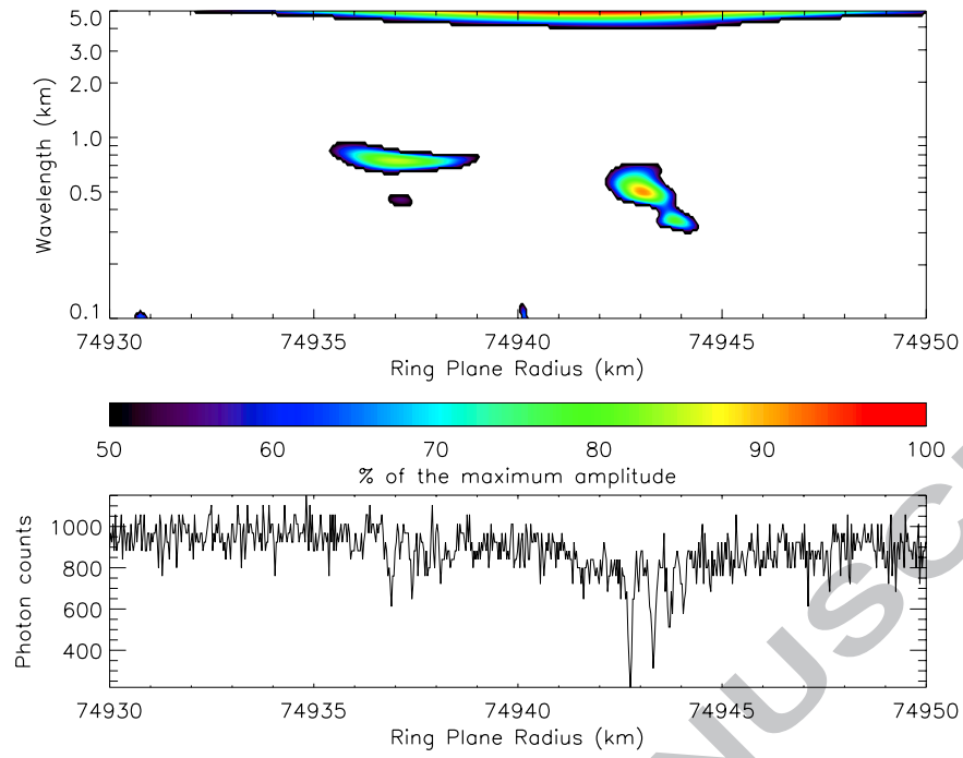
Figure 16. WWZ wavelet power profile of structures 3 and 4, computed from \alpha Virginis, rev. 30 individual occultation profile.
