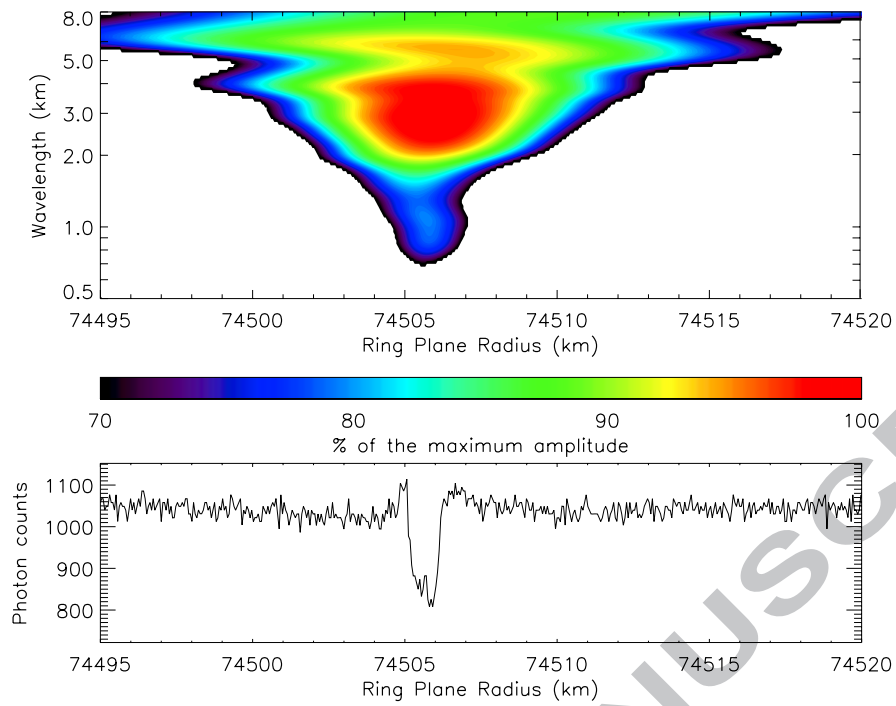
Figure 3. WWZ wavelet power profile of embedded ringlet ER1 computed from 62 individual occultation profiles. Lower panel shows the \beta Centauri, rev. 85 occultation profile. Embedded ringlets produce this characteristic triangular profile in the power contour plots.
