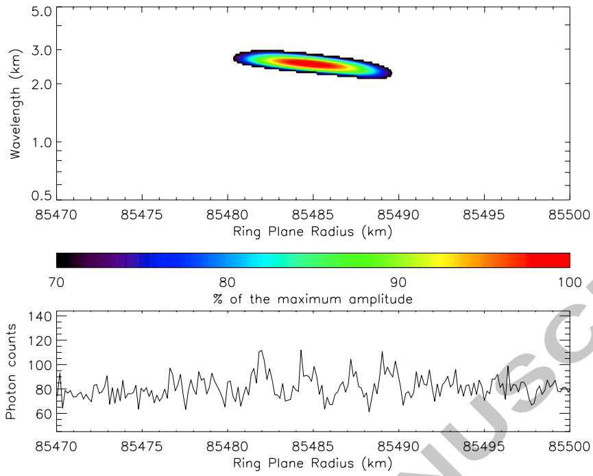
Figure 19. WWZ wavelet power profile of structure 24, computed from \zeta Orionis, rev. 47 individual occultation profile. Feature 24 is located between plateaus P5 and P6.
