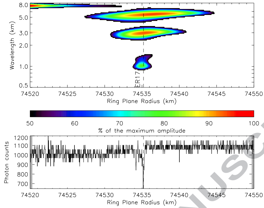
Figure 6. Co-added WWZ wavelet power profile of embedded ringlet ER17, computed from individual occultation profiles. Lower panel shows the \alpha Virginis, rev. 30 occultation profile. A clear triangular shape is visible as the resulting signature of embedded ringlet ER17.
