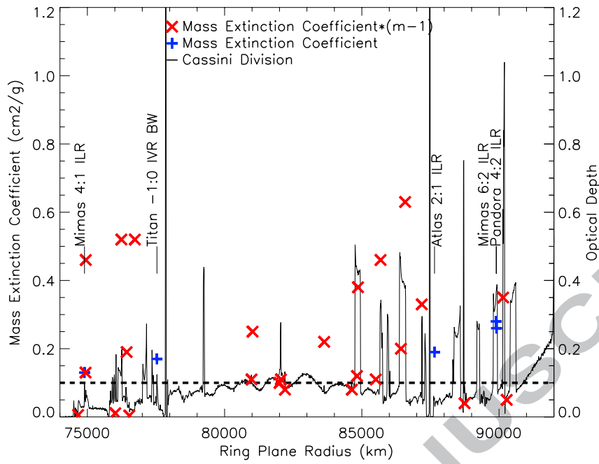
Figure 32. Mass extinction coefficient limit values. Actual mass extinction coefficient values, calculated at the associated resonance locations, are displayed in blue while upper limits of mass extinction coefficient, estimated from \kappa \times (m - 1) , are shown in red.
