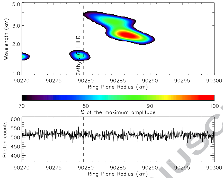
Figure 24. WWZ wavelet power profile of wave 40, computed from \beta Centauri, rev. 81 individual occultation profile. Tethys 6:1 ILR is at 90279.6 km (vertical dashed line). Its calculated strength is very low, suggesting that this is a chance association (Tiscareno et al. (2007)). Wave source location is outside the range of this figure, at 90238.5 \pm 2.5 km.
