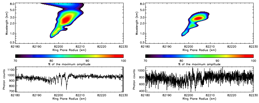
Figure 27. WWZ wavelet power profile of structure 17, computed from co-added wavelet profiles of high-incidence angle occultations (left) and low-incidence angle occultations (right). Lower panel show the \beta Centauri, rev. 85 occultation profile (left) and the \alpha Virginis, rev. 34 occultation profile (right).
