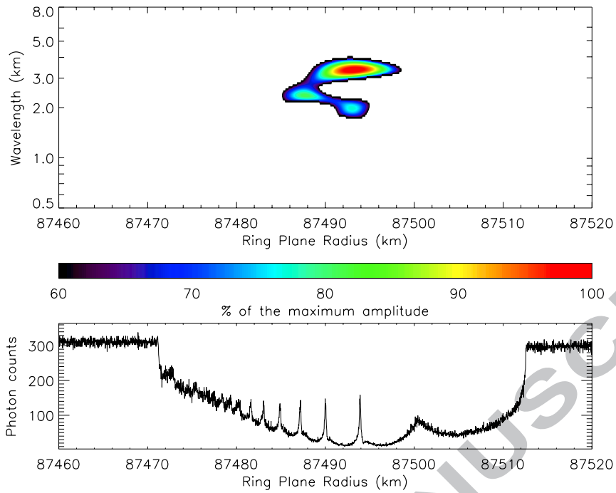
Figure 29. WWZ wavelet power profile around Maxwell ringlet, computed from \beta Centauri, rev. 105 individual occultation profile. Though the structure is quite clear and prominent to the eye on the occultation profile, the WWZ profile is distorted by the relative importance of the amplitude of the highest wavelengths, hiding smaller amplitudes at the presented scale.
