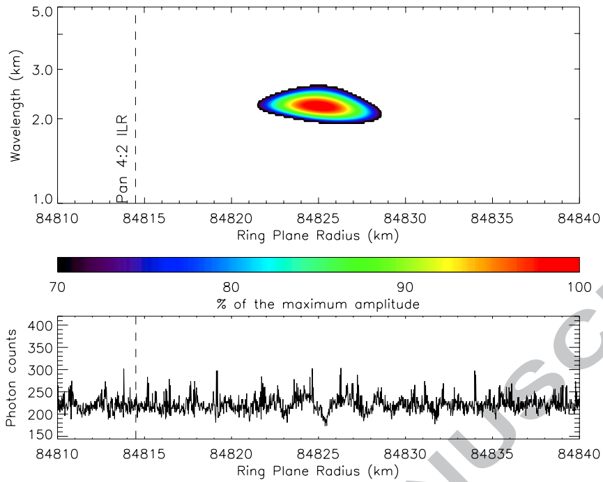
Figure 22. WWZ wavelet power profile of feature 20, computed from \beta Centauri, rev. 104 individual occultation profile. Pan 4:2 ILR is at 84814.5 km (vertical dashed line). The relatively long distance between the Pan 4:2 ILR and the wave (about the same distance as the length of the wave itself) together with a very low torque value for this resonance and an inconsistent wave source location from the feature invalidate the possibility of an association. Wave source location is outside the range of this figure, at 84775 \pm 8 km.
