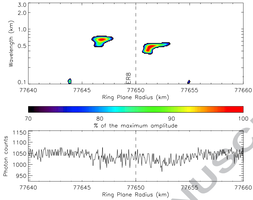
Figure 5. Co-added WWZ wavelet power profile of embedded ringlet ER8, computed from individual occultation profiles. Lower panel shows the \beta Centauri, rev. 85 occultation profile. The double peaks, characteristic of ER8, present clear signatures.
