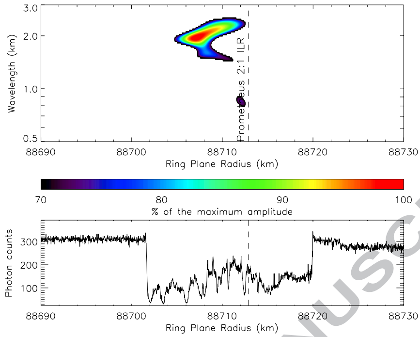
Figure 15. WWZ wavelet power profile of R4 ringlet, computed from \beta Centauri, rev. 105 individual occultation profile. The Prometheus 2:1 ILR position is represented by a vertical dashed line.
