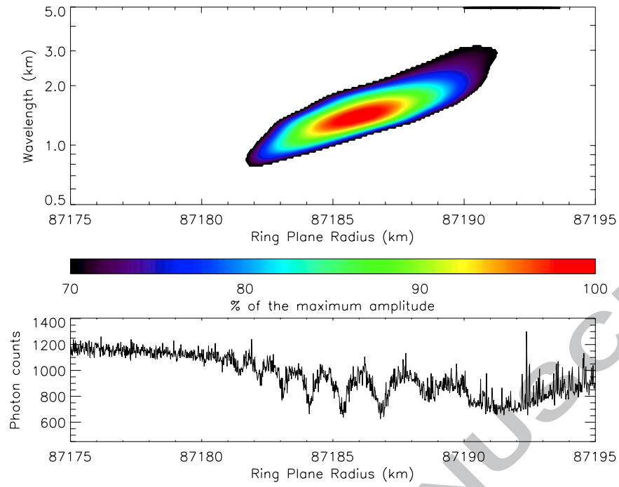
Figure 9. Co-added WWZ wavelet power profile of structure 32, computed from individual occultation profiles. Lower panel shows the \beta Centauri, rev. 85 occultation profile. Structure 32 is coexisting with the embedded ringlet ER13 that spreads from 87180 km to 87210 km.
