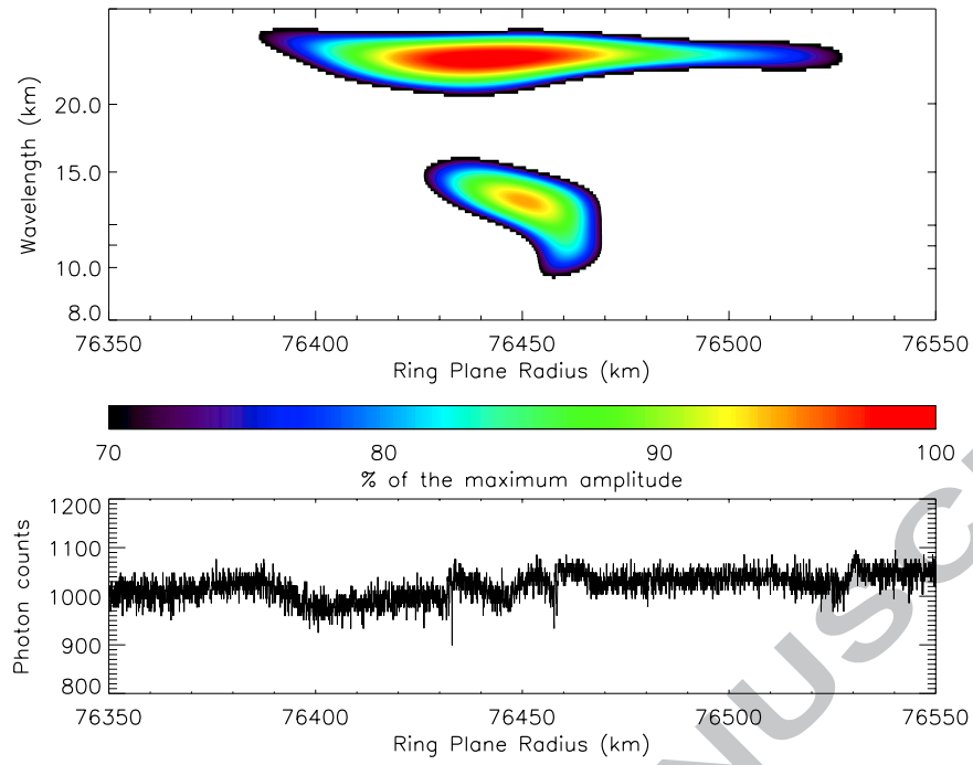
Figure 17. WWZ wavelet power profile computed from \beta Centauri, rev. 85 individual occultation profile showing structures 7 and 8 coexisting at the same location. Figure 18 gives more details about the central region where structure 9 is located.
