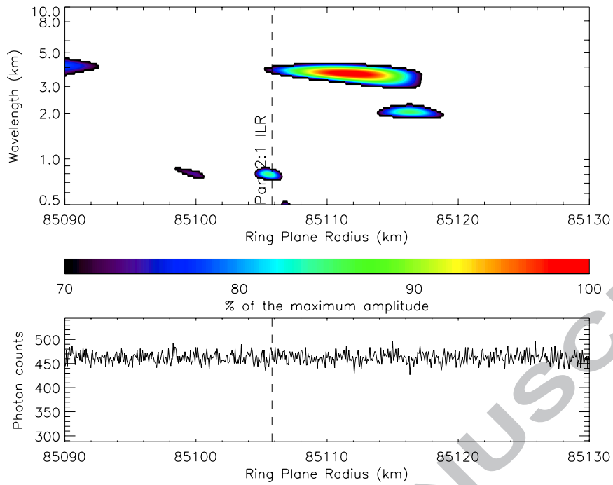
Figure 23. WWZ wavelet power profile of structure 22, computed from \beta Centauri, rev. 89 individual occultation profile. Pan 2:1 ILR is at 85105.8 km (vertical dashed line). No obvious direction of propagation can be determined from diverse occultations. Wave source location is outside the range of this figure, at 84989 \pm 20 km.
