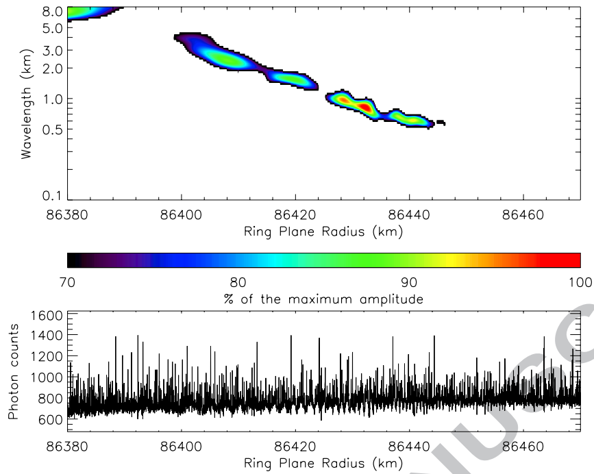
Figure 21. Co-added WWZ wavelet power profile of structure 28, computed from individual occultation profiles. Lower panel shows the \beta Centauri, rev. 89 occultation profile. Structure 28 is one of the most extended feature observed in the C ring, but there is no low order resonance in its vicinity.
