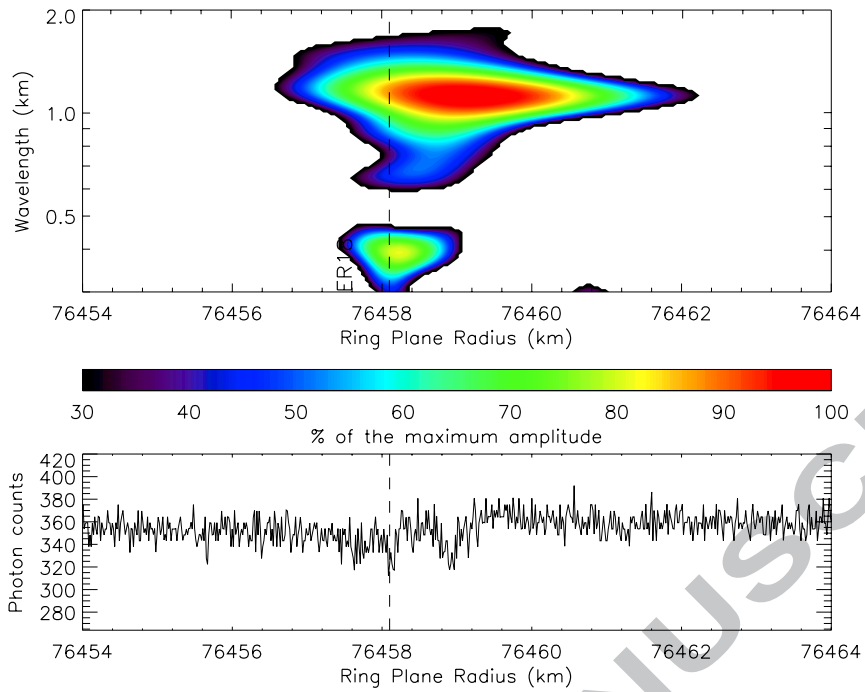
Figure 7. Co-added WWZ wavelet power profile of embedded ringlet ER18, computed from individual occultation profiles. Lower panel shows the \beta Centauri, rev. 104 occultation profile. Two peaks, separated by 0.8 km, are visible on the occultation profile.
