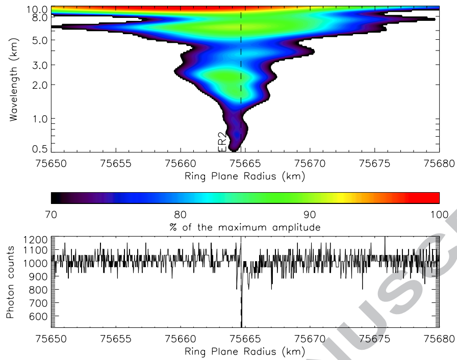
Figure 4. Co-added WWZ wavelet power profile of embedded ringlet ER2, computed from individual occultation profiles. Lower panel shows the \alpha Virginis, rev. 34 occultation profile. A clear triangular shape is visible as the resulting signature of embedded ringlet ER2.
