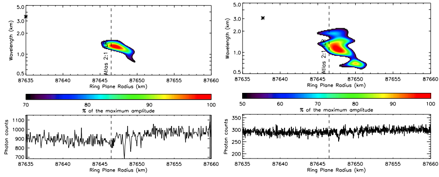
Figure 13. WWZ wavelet power profile of wave 33, computed from \alpha Virginis, rev. 34 (left) and \beta Centauri, rev. 105 (right) individual occultation profiles. The Atlas 2:1 ILR (at 87646.5 km - vertical dashed line) has a greater torque than the Pan 2:1 ILR which does not seem to excite a wave at 85105 km. The asterisks locate the positions of the observed wave sources. Profiles of this wave consistently show a dispersion that places the wave source several km interior to the wave feature and the theoretical location of the Atlas 2:1 ILR.
