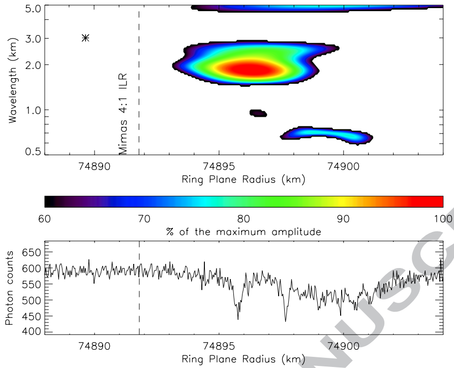
Figure 11. WWZ wavelet power profile around the Mimas 4:1 inner Lindblad resonance ( r_L = 74891.9 km, marked by the vertical dashed line), computed from \beta Centauri, rev. 75 individual occultation profile. The possible superposition with a ringlet structure is disturbing our perception of the direction of propagation. The asterisk locates the position of the observed wave source.
