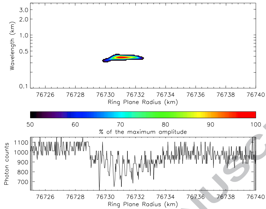
Figure 28. WWZ wavelet power profile of structure 11, computed from \alpha Virginis, rev. 30 individual occultation profile.
