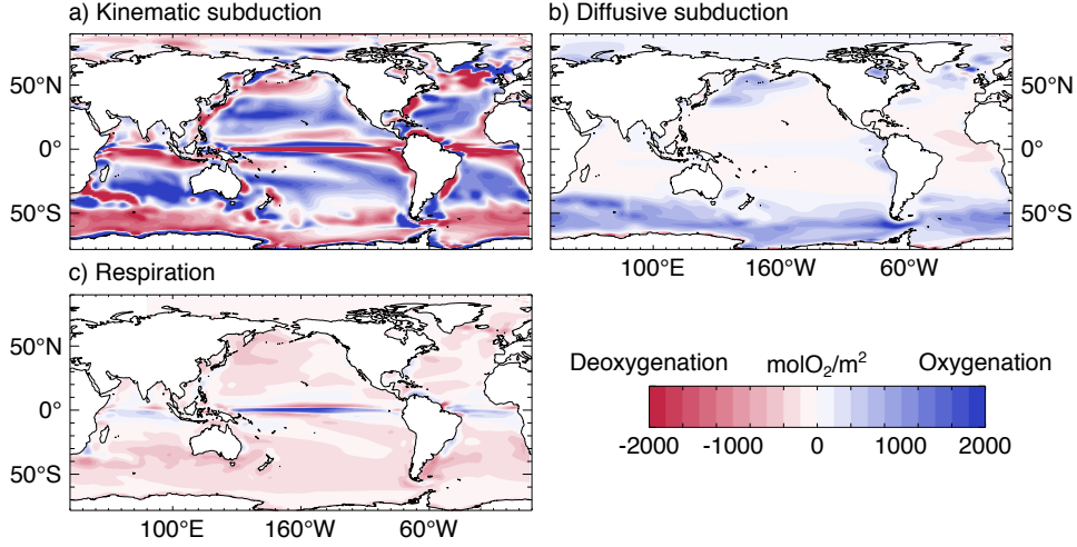
Figure 1. Spatial patterns of a) kinematic oxygen subduction ( S_{kin} ), b) diffusive oxygen subduction ( S_{mix} ) and c) respiration ( R ) in the CTL simulation, cumulated over a period of 110 years, from 1990 until 2099. A Gaussian blur has been applied before plotting to smooth grid-point noise.
