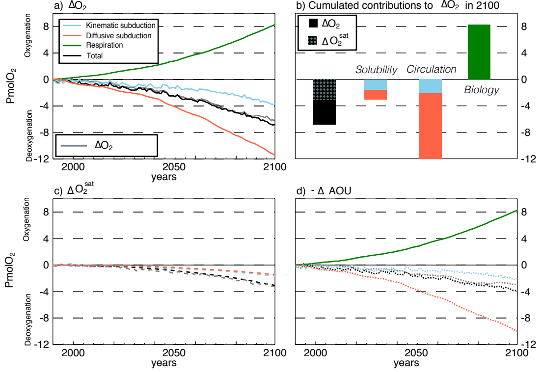
Figure 3. Factors explaining global deoxygenation along the 21st century in the IPSL-CM5A-LR projection under scenario RCP8.5. a) Time cumulated evolution of kinematic subduction ( \Delta\hat{S}_{kin} , blue line), diffusive subduction ( \Delta\hat{S}_{mix} , red line), respiration ( \Delta\hat{R} , green line), their sum (Total, black line) and changes in subsurface O_2 ( \Delta\hat{O}_2 , grey line) integrated over the global ocean. c) Same for changes due to solubility ( \Delta\hat{S}_{kin}^{sol} and \Delta\hat{S}_{mix}^{sol} , dashed blue and red lines with their sum in dashed black) compared to changes in O_2^{sat} ( \Delta\hat{O}_2^{sat} , dashed grey line). d) Same for changes due to circulation ( \Delta\hat{S}_{kin}^{circ} and \Delta\hat{S}_{mix}^{circ} , dotted blue and red lines) and respiration ( \Delta\hat{R} , green line), with the sum of the three in dotted black, compared to changes in AOU ( -\Delta AOU , dotted grey line). b) Time cumulated contributions to global deoxygenation in 2100, sorted by solubility ( \Delta\hat{S}_{mix}^{sol} and \Delta\hat{S}_{kin}^{sol} ), circulation ( \Delta\hat{S}_{mix}^{circ} and \Delta\hat{S}_{kin}^{circ} ) and biology ( \Delta\hat{R} ), compared to global deoxygenation ( \Delta\hat{O}_2 ) and \Delta\hat{O}_2^{sat} .
