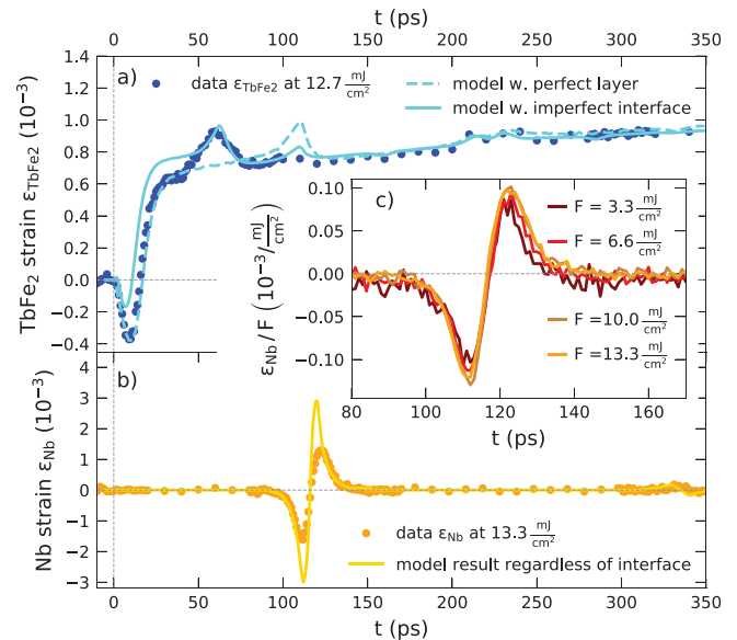
FIG. 2. Transient strain signatures of sample 1 without \text{SiO}_2 capping: (a) and (b) display transient strains extracted from the average peak shift via Gaussian line-shape fits and the simulated strain response using the udkm1Dsim toolbox as lines. The dashed line in (a) corresponds to a model with a full single-crystalline \text{TbFe}_2 layer whereas the solid line takes a disordered \text{TbFe}_2 layer at the \text{TbFe}_2/\text{Nb} interface into account. Inset (c) depicts the transient strain pulse in the \text{Nb} layer normalized to the different excitation fluences.
