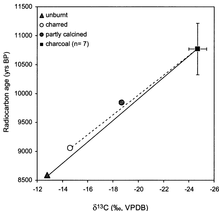
Figure 4 ^{14}\text{C} ages versus \delta^{13}\text{C} values of charcoal and pig bone apatite from Akrotiri-Aetokremnos (Cyprus). Data can be found in Simmons (1999) and Vigne et al. (2009).
