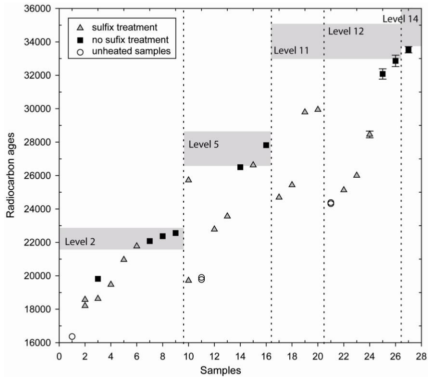
Figure 4 Comparison between ^{14}\text{C} ages obtained on unburned and calcined bones at Abri Pataud and expected ages for the corresponding levels. Expected age boundaries are based on recently published dates obtained on bone collagen (Higham et al. 2011; Henry Gambier et al. 2013).
