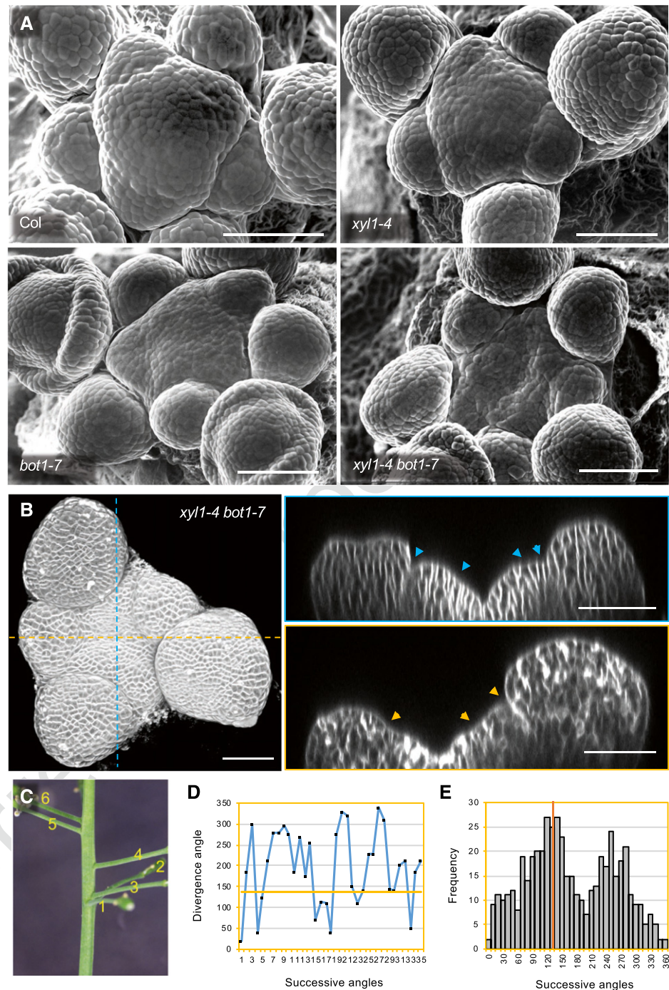
Figure 9. Phenotype of xy1-4 bot1-7 . A, Scanning Electron Microscope (SEM) images of Col, xy1-4 , bot1-7 , and xy1-4 bot1-7 SAMs. B, Three dimensional reconstruction (left) and orthogonal view (right) of confocal image of xy1-4 bot1-7 meristem. The arrow-heads mark the points with negative curvatures on meristem surface, which are proposed to be organ boundaries. Scale bars = 50 \mu m (A and B). C, Representative image of silique distribution on xy1-4 bot1-7 stem. Numbers denote the silique positions from bottom to top (old to young). D, Representative silique distribution angles on the inflorescence stem of xy1-4 bot1-7 . E, Distribution of divergence angles of siliques on the xy1-4 bot1-7 inflorescence stems. Orange line denotes the position of angle around 137°; n = 504 angles from 10 plants.
