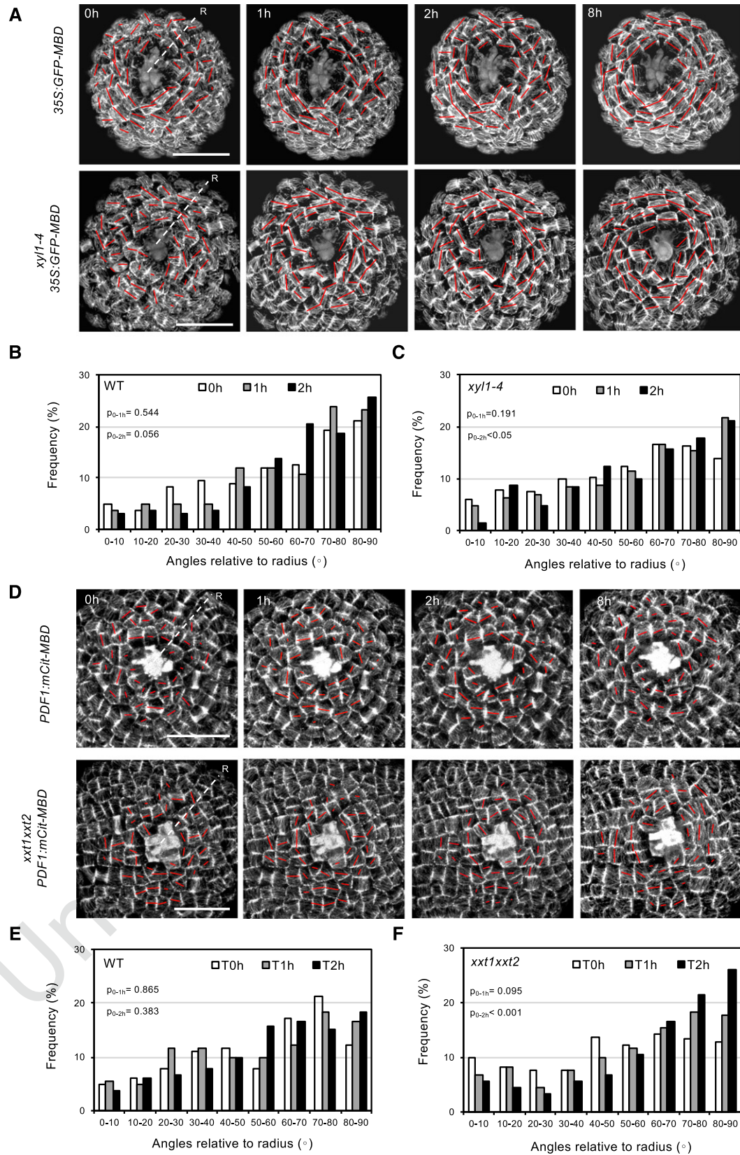
Figure 8. CMT reactions to mechanical perturbation in wild-type, xy1-4 , and xxt1xxt2 SAMs. A, Time series of CMT patterning in 35S::GFP-MBD (wild type [WT]) and xy1-4 35S::GFP-MBD SAMs after laser ablation at the meristem center. The orientation and
