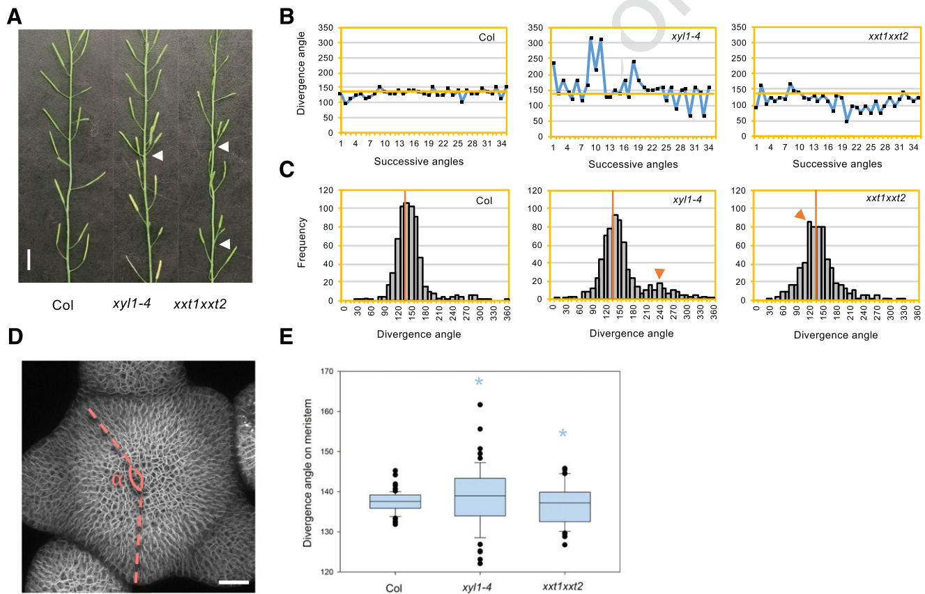
Figure 4. Phyllotactic phenotype of XyG mutants. A, Representative image showing perturbation of phyllotaxis (indicated by arrowhead) in xy11-4 and xtt1xtt2 mutants. Scale bar = 1 cm. B, Representative distribution angles of siliques on the inflorescence stem of Col, xy11-4 , and xtt1xtt2 plants. C, Distribution of divergence angles of siliques on the Col, xy11-4 , and xtt1xtt2 inflorescence stems. Orange lines denote the position of a divergence angle of 137°. Orange arrowheads mark the abnormal angle peaks; n = 649 angles from 20 Col plants; n = 683 angles from 21 xy11-4 plants; n = 635 angles from 21 xtt1xtt2 plants. D, Diagram showing the method to measure the divergence angles ( \alpha ) between successive primordia on confocal images of live meristems. Scale bar = 20 \mu\text{m} . E, Primordia distribution angles on Col, xy11-4 , and xtt1xtt2 meristems; n = 67 angles from 11 Col meristems; n = 55 angles from 6 xy11-4 meristems; n = 46 angles from 8 xtt1xtt2 meristems. Asterisks denote statistically significant differences with wild type; *P < 0.05 , Kolmogorov-Smirnov test.
