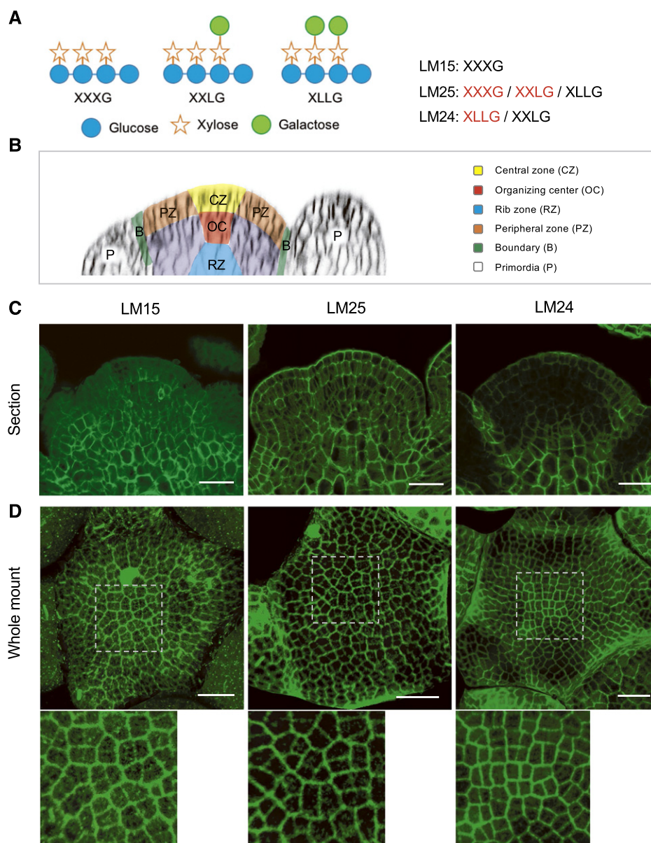
Figure 1. Differential distribution of xyloglucans (XyGs) in Arabidopsis wild-type shoot apices. A, Schematic structures of XyG subunits and specificity of XyG antibodies. Letters highlighted by red color mean higher affinity. B, Schematic structure of Arabidopsis SAM. C and D, Immunolocalization of XyGs in wild-type (Col) shoot apex sections (C) and whole mount tissues (D) labeled with LM15, LM25, and LM24 antibodies. Details are shown at bottom of (D). Scale bars = 20 \mu\text{m} .
