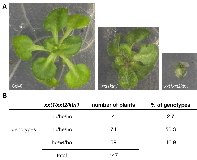
Figure 10. Phenotype of a triple mutant xxt1xxt2ktn1 . A, Phenotype of representative Col-0, xxt1ktn1 , and xxt1xxt2ktn1 plants grown in vitro for 3 weeks. Scale bar = 1 mm. B, Analysis of the progeny a xxt1 -/- xxt2 +/- ktn -/- plant. Among 147 plants, we identified 4 triple mutants.
