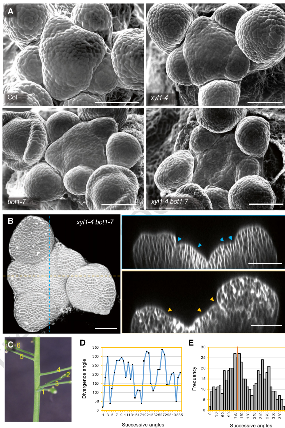
Figure 9. Phenotype of xy11-4 bot1-7 .
