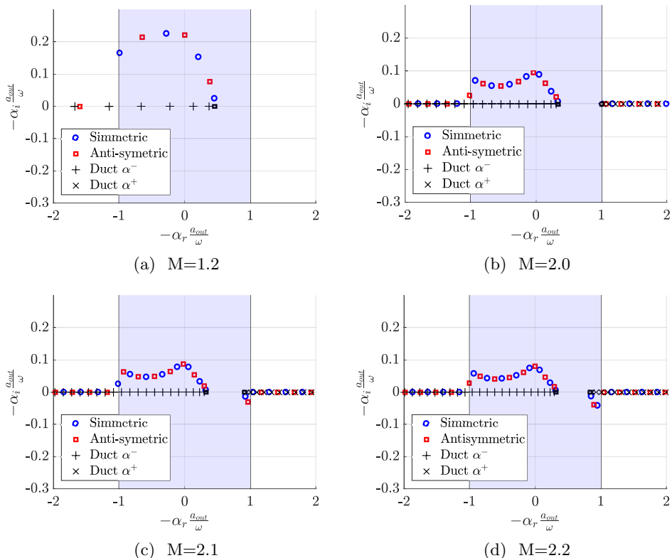
Figure 17: Instability of supersonic \alpha^+ and stability of supersonic \alpha^- modes for a left pointing jet. Results are plotted in terms of -\alpha . All subsonic modes are neutrally stable, all supersonic modes being either stable ( -\alpha_i > 0 ) or unstable ( -\alpha_i < 0 ). Coloured markers indicate DVS modes, black markers indicated duct modes, with the n = 0 mode identified by a square marker: this mode is not present in the soft-walled limit, appearing only at the transition to hard-walled behaviour. The blue region indicates supersonic phase speeds with respect to the outer region. Mach numbers 1.2, 2.0, 2.1, 2.2 from left to right, top to bottom. The plot is for constant Helmholtz numbers, \omega = \pi , and \rho_r = T_r = 1 .
