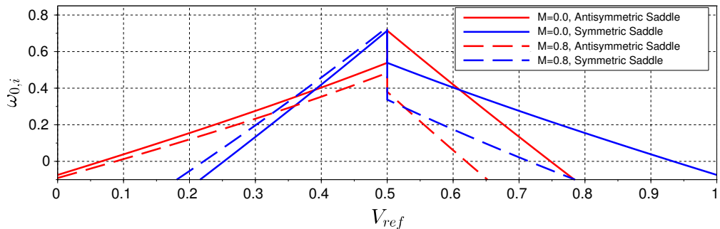
Figure 19: Growth rates of pseudo wave-packets of the DVS flow, for T_r = 1 .
