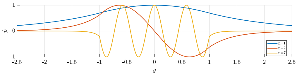
Figure 18: Pressure support for the first, second and seventh \alpha^+ duct-like modes in a M = 2.0 jet. Lower harmonics, which have near-sonic phase velocities with respect to the outer flow, resemble hard-walled duct modes; a transition to soft-duct behaviour is observed as the harmonic number increases. Results are for V_{ref} = 1 and \omega = \pi .
