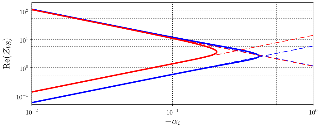
Figure 15: Relation between real part of impedance and \alpha_i for the upstream-travelling modes of figure 13. Solid lines indicate dispersion-relation solutions, equation 2.11, and dashed lines show the first-order correction provided by equation 4.20.
