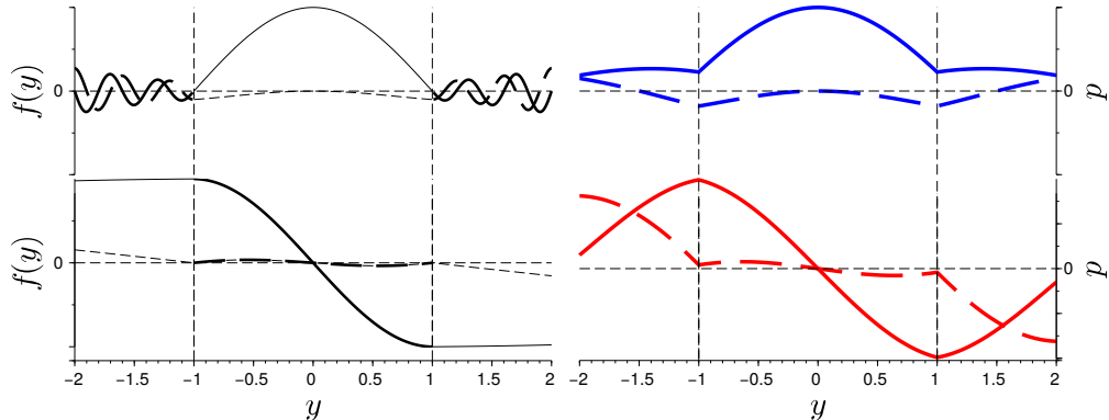
Figure 11: Analogy with vibration of an infinite string with DVS modes exhibiting discontinuous density and pressure. The left plot shows an infinite, vibrating string with discontinuous density, the thick line indicating higher density. The right plots show duct-like modes of the jet (top) and the wake (bottom) for \omega = 0.8 . Solid and dashed lines indicate the real and imaginary parts of the eigenfunctions, respectively.
