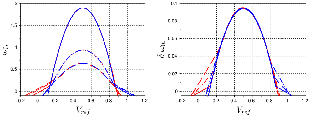
Figure 21: Wave-packets growth rates for \delta = 0.05, 0.10 and 0.20 (solid, dashed and dotted lines, respectively). Blue and red lines correspond to symmetric and antisymmetric modes, respectively. (a) Growth rates based on shear-layer separation; (b) Growth rates rescaled using the shear-layer thickness \delta .
