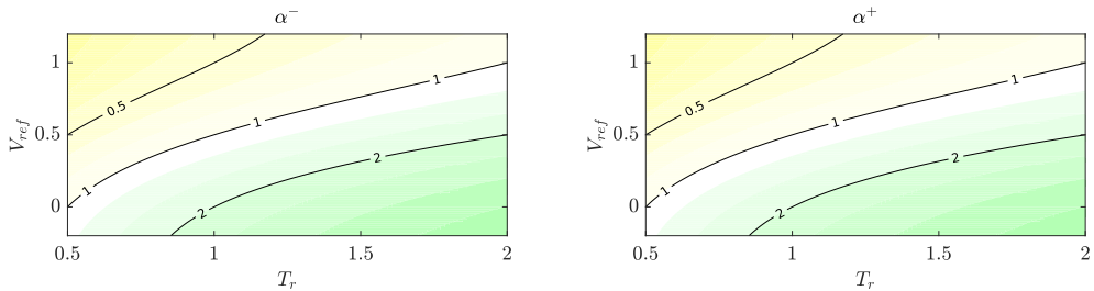
Figure 7: Impedance-ratio ( Z_{VS}/Z_{ref} ) map showing dependence on T_r and V_{ref} . Colour map is the same as in Figure 5, for \rho_r = 1, \omega = \pi/2, M = 0.01 , for the first harmonic duct mode ( n = 1 ).
