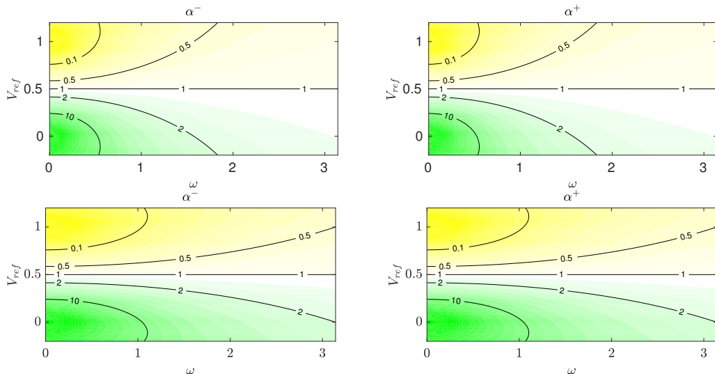
Figure 5: Impedance-ratio map indicating regions where modes resemble those of soft- (yellow) or hard-walled (green) acoustic ducts. A clear trend is identified at low frequency, wakes ( V_{ref} < 0.5 ) and jets ( V_{ref} > 0.5 ) exhibiting hard- and soft-walled behaviours, respectively. The distinction deteriorates at higher frequencies. The colour scale corresponds to absolute value of the impedance ratio ( Z_{VS}/Z_{ref} ) for T_r = 1, \rho_r = 1, M = 0.01 . Top and bottom plots correspond, respectively, to first ( n = 1 ) and second ( n = 2 ) harmonic, duct-like modes.
