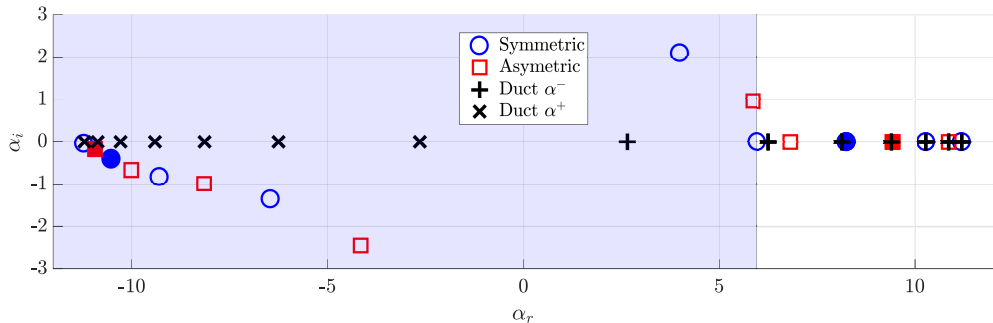
Figure 13: Roots of Equation 2.11 for V_{ref} = 0 , M = 0.9 , \rho_{in,out} = 1 , and \omega = 4\pi . Blue and red markers indicate symmetric and asymmetric modes, respectively, solid circles indicate the modes considered in figures 14 and 15. Hard- and soft-walled duct roots are indicated by “x” and “+”, respectively. The blue region indicates supersonic phase-velocity with respect to the outer flow.
