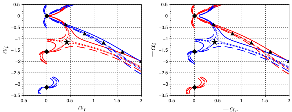
Figure 9: Same as Figure 8, but with saddle point formed due to changes in V_{ref} . Solid, dotted, and dashed lines corresponds to V_{ref} = (1.00, 0.95, 0.93, 0.90) for the jet and (0.00, 0.06, 0.07, 0.10) for the wake. Neutral saddles (black stars), are found for V_{ref} = 0.935 and 0.065 for the jet and wake, respectively.
