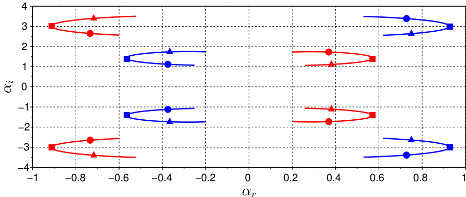
Figure 23: Locus of eight DVS saddle point with increasing V_{ref} . Symmetric and antisymmetric mode saddles in red and blue. The triangle, square and circle markers correspond to V_{ref} = 0, 0.5 and 1.0 .
