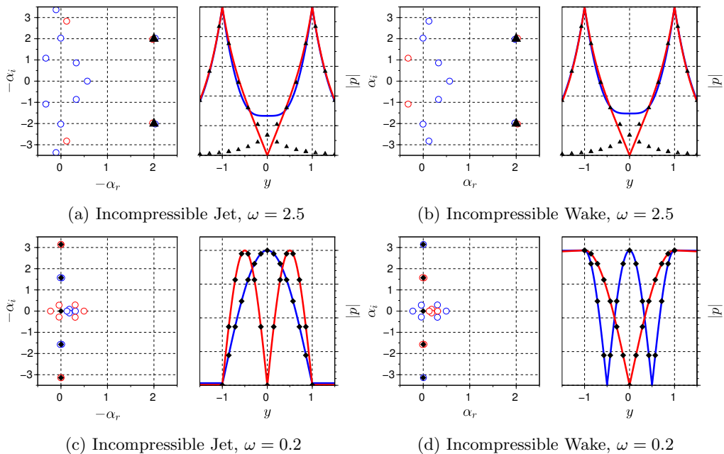
Figure 4: Comparison between DVS and KH modes (top) and duct-like modes (bottom). Spatial spectra are shown on the left of each sub plot, with blue and red circles indicating symmetric and antisymmetric DVS modes, respectively, black diamonds acoustic-duct modes and triangles single vortex-sheet KH modes. The right-hand sub plots show eigenmode comparisons between DVS (solid lines), acoustic-duct modes (diamonds) and single vortex-sheet KH modes (triangles).
