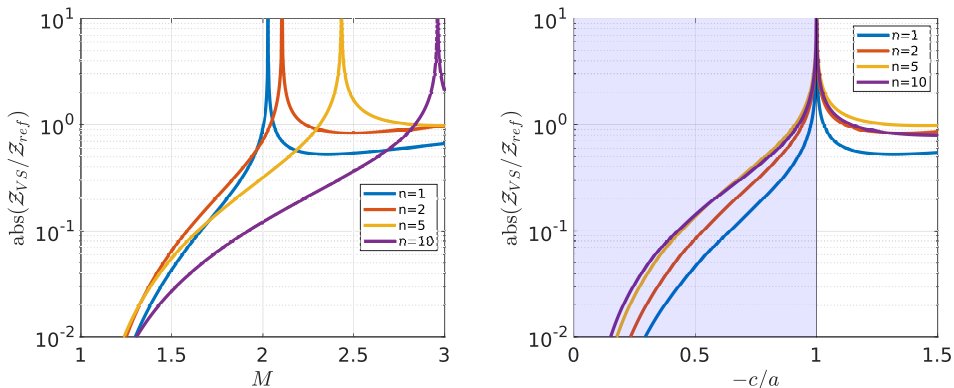
Figure 16: Absolute values of impedance for \alpha^+ duct modes as a function of Mach number (left) and of duct-mode phase speed (right). Impedance peaks, found at different M for each harmonic, occur when the phase speed of the mode is sonic. Results are for \omega = \pi , with the blue region indicating subsonic phase-speeds.
