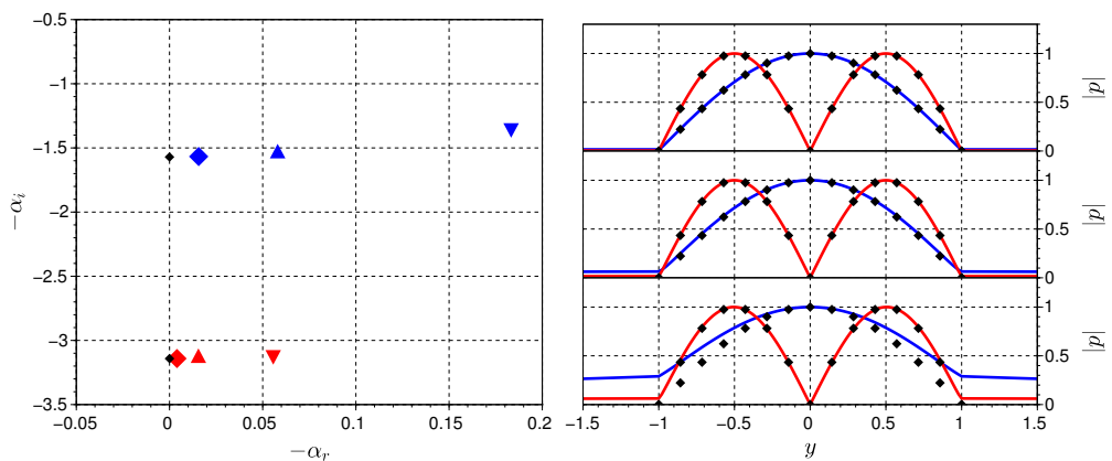
Figure 6: Deviation of DVS jet ( V_{ref} = 1 ) modes from acoustic, duct-like behaviour with increasing frequency. Left plot shows DVS, the markers \diamond, \triangle, \nabla indicating, respectively \omega = 0.2, 0.4 and 0.8 ; the right plot shows corresponding pressure eigenfunctions, for, from top to bottom, \omega = 0.2, 0.4 and 0.8 , black diamonds indicating the corresponding acoustic-duct mode.
