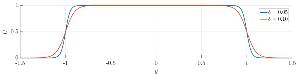
Figure 20: Illustration of a finite shear-layer jet obtained with Equation 5.2.
