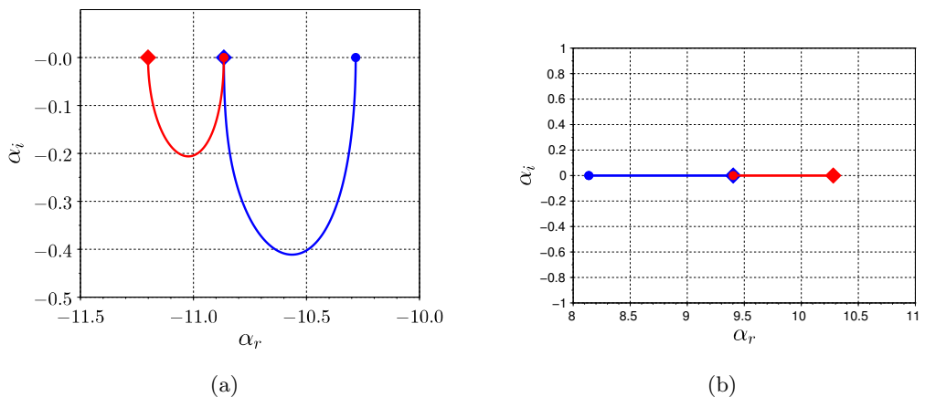
Figure 14: Loci, as a function of \rho_r , of upstream- (left) and downstream- (right) travelling modes, indicated in the left and right half planes of figure 13. Upstream-travelling modes move in to the complex \alpha plane, while downstream-travelling modes remain on the real axis due to total reflection. Limits of hard- ( \rho_r = \infty ) and soft-duct ( \rho_r = 0 ) behaviour are indicated, respectively, by diamonds and circles. Red and blue lines represent antisymmetric and symmetric modes, respectively.
