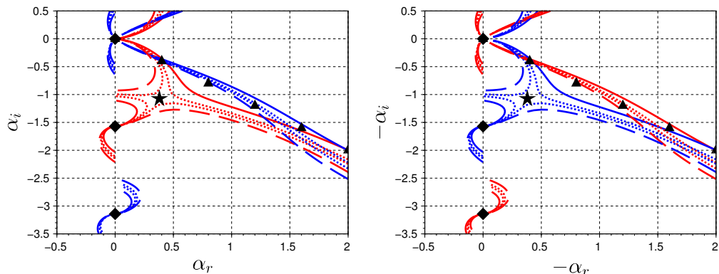
Figure 8: Spatial eigenspectra for incompressible ( M = 0.01 ) wake (left) and jet (right), showing “pinching” of the acoustic and KH branches with temperature variation. Solid, dotted, and dashed lines corresponds to T_r of (1.00, 0.83, 0.76, 0.66) on the left and (1.0, 1.2, 1, 3, 1.5) on the right. Blue/red lines indicate antisymmetric/symmetric modes, diamonds/triangles indicate duct/KH modes. Neutral saddles location with real \omega_0 are found at T_r \approx 1.26 for the jet and at T_r \approx 0.79 for the wake (black stars). Loci are shown for \omega \in [0, 1.5\pi] .
