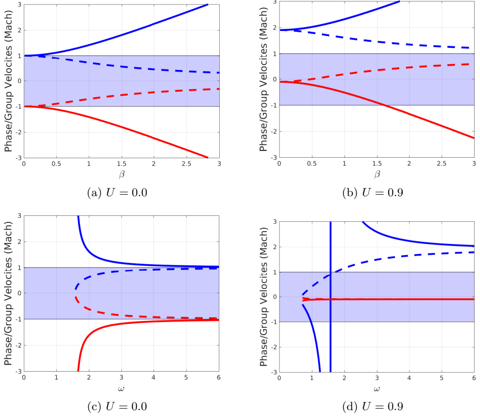
Figure 22: Behavior of phase (solid) and group (dashed) velocities for the positive (red) and negative (blue) signs for propagative modes. Shaded regions indicates the subsonic velocities on the laboratory reference frame. For figures (a) and (b) a = 1 , \omega = 1 and \alpha(\omega, \beta) , while for (c) and (d) a = 1 and \beta = \pi/2 were used, with \omega(\alpha, \beta) . The interdependency of \alpha, \beta, \omega are given by equation A 3. Note that the boundary conditions limit the allowable values of \beta to multiples of \pi/2 , nevertheless we keep all values of \beta for a clearer visualization of the trends.
