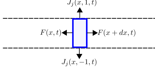
Figure 12: Schematic depiction of energy balance analysis. Control volume shown in blue, vortex-sheets indicated by the black dashed lines and energy fluxes by arrows.
