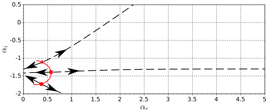
Figure 24: Briggs criteria for 4th quadrant saddle points for different V_{ref} . Red line represents the saddle point locus, black dashed lines show the path for both of the saddle roots with increasing \omega_i , with arrows indicating direction of increasing \omega_i .
