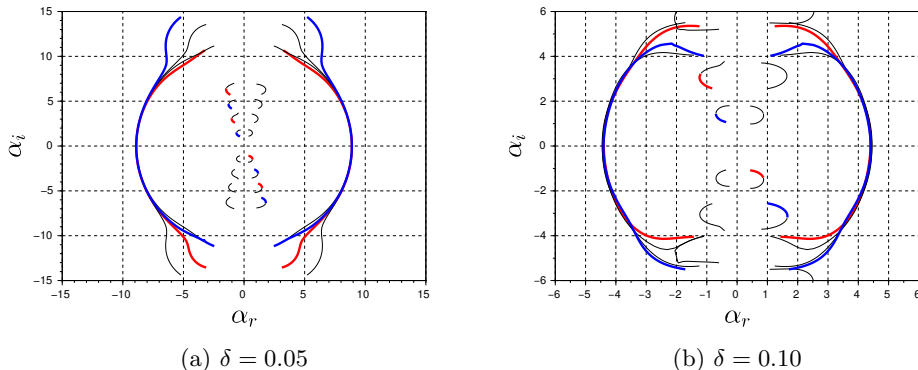
Figure 25: Saddle locus in the complex \alpha -plane with V_{ref} . Blue and red lines indicate “valid” (saddle formed by upstream- and downstream-traveling modes) symmetric and antisymmetric modes. Black lines indicate invalid saddles. For small values of \delta there is a clear distinction between columns and shear layer saddles.
