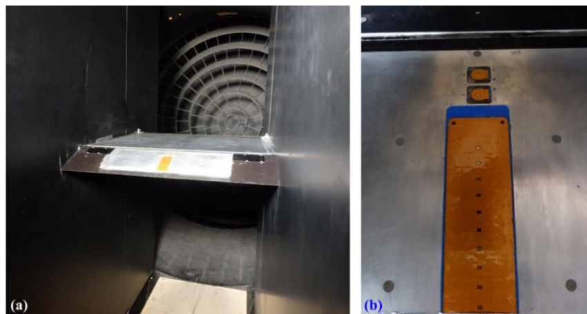
Figure 6: (a) Flap model with implemented micro-sensors (b) Zoom on the twelve micro-sensors: two individual sensors at the leading edge and a strip of ten sensors with shared electronics
