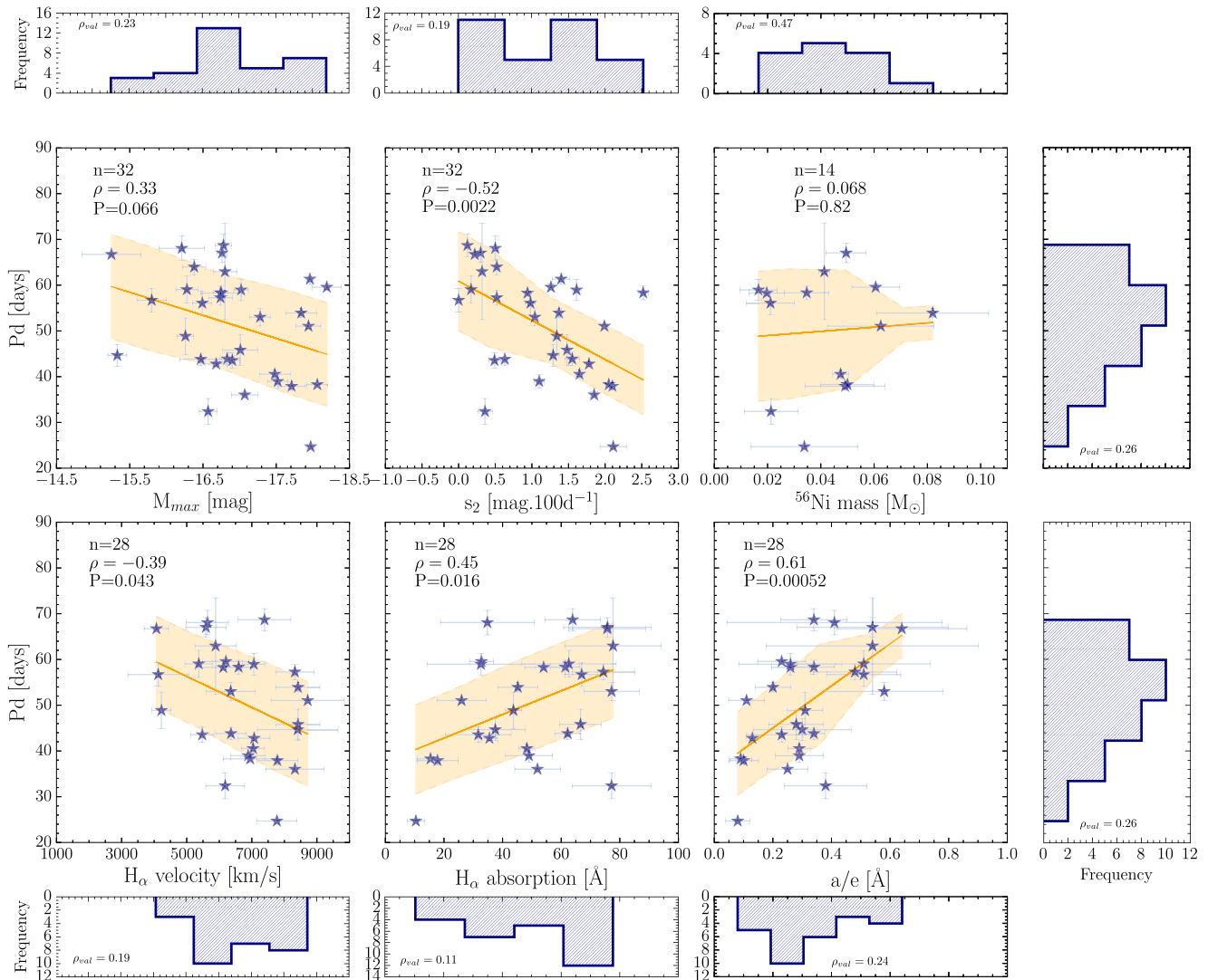
Figure 10. Correlations between Pd and six different parameters: M_{\max} , s_2 , ^{56}\text{Ni} mass, H_\alpha velocity, pEW of H_\alpha absorption component, a/e . On the top of the figure, n = number of events, \rho = Pearson's correlation coefficient, and P = probability of detecting a correlation by chance. In addition, each plot shows the corresponding best fit ( linmix_err ; Kelly 2007) as a solid orange line, while the orange shaded area indicates the variance with respect to the fit line. Histograms along the x- and y-axes show the distributions of the various parameters plotted on each axis. Each histogram displays the \rho_{\text{val}} found using the Shapiro–Wilk normalization. When the \rho_{\text{val}} > 0.05 , the data set comes from a population that has a normal distribution.
