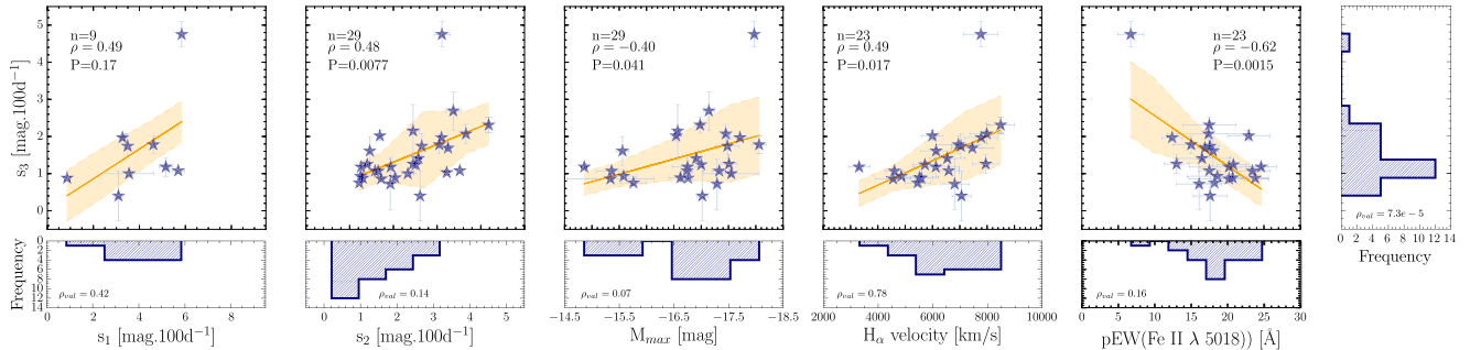
Figure 14. Correlations between s_3 and five different parameters: s_1 , s_2 , M_{\max} , H_{\alpha} velocity, pEW(Fe II \lambda 5018). On the top of the figure, n = number of events, \rho = Pearson's correlation coefficient, and P = probability of detecting a correlation by chance. Histograms along the x- and y-axes show the distributions of the various parameters plotted on each axis. Each histogram displays the \rho_{\text{val}} found using the Shapiro–Wilk normalization. When the \rho_{\text{val}} > 0.05 , the data set comes from a population that has a normal distribution.
