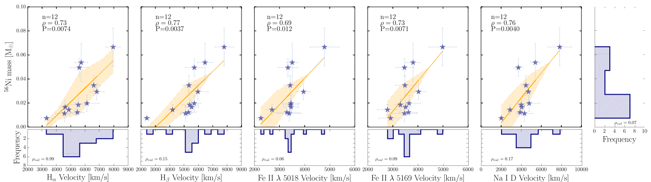
Figure 12. Correlations between ^{56}\text{Ni} and the expansion velocities. On the top of the figure, n = number of events, \rho = Pearson's correlation coefficient, and P = probability of detecting a correlation by chance. In addition, each plot shows the corresponding best fit ( linmix_err ; Kelly 2007) as a solid orange line, while the orange shaded area indicates the variance with respect to the fit line. Histograms along the x- and y-axes show the distributions of the various parameters plotted on each axis. Each histogram displays the \rho_{\text{val}} found using the Shapiro–Wilk normalization. When the \rho_{\text{val}} > 0.05 , the data set comes from a population that has a normal distribution.
