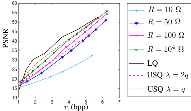
Fig. 7: Comparison between (i) the Dual-SIMQ, (ii) the USQ with deazone \lambda = q , (iii) the USQ without deadzone ( \lambda = 2q ) and (iv) the non-uniform Lloyd quantizer for 100 synthetic normal zero mean distribution signals (set of parameters: C = 1 F, T = 150 ms, \theta \in \{1, R, \dots, 10R\} V, \lambda = q , q = \{1, 8, 10, 15, 20, 40, 60, 80, 100\} ).
