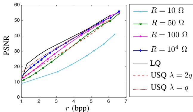
Fig. 10: Comparison between (i) the Dual-SIMQ, (ii) the USQ with deazone \lambda = q , (iii) the USQ without deadzone ( \lambda = 2q ) and (iv) the non-uniform Lloyd quantizer for 100 real images taken from [31] (set of parameters: C = 1 F, T = 150 ms, \theta \in \{1, R, \dots, 10R\} V, \lambda = q , q = \{1, 8, 10, 15, 20, 40, 60, 80, 100\} ).
