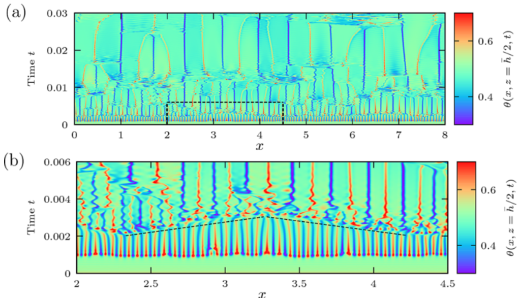
FIGURE 6. Spatio-temporal evolution of the temperature at the middle of the fluid layer \theta(x, \bar{h}/2, t) . (a) Full duration of the simulation 0 < t < 3 \times 10^{-2} and full spatial extent 0 < x < 8 . The dashed line corresponds to the zoom shown below. (b) Zoom in at early times 0 < t < 6 \times 10^{-3} , the dashed lines follow the propagation of a defect in the initially-steady array of convective rolls.
