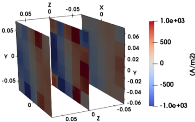
(c) Air stoichiometry = 1.3
