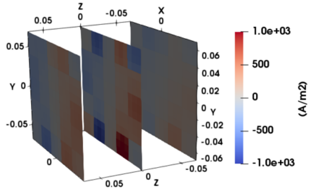
(b) Air stoichiometry = 1.5
