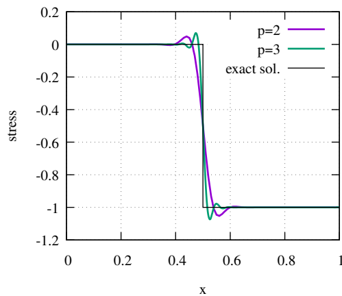
Figure 1: Bar impact: normalized compressive stress upon the position along the bar at t=0.5s
