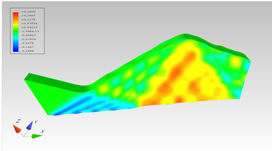
Figure 2: Impact of a plane strain elastic beam-like structures: x axis corresponds to time, y and z to space. Isocolor of the first component of the kinematic field. Non stabilized solution.
