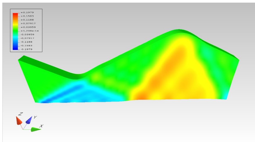
Figure 3: Impact of a plane strain elastic beam-like structures: x axis corresponds to time, y and z to space. Isocolor of the first component of the kinematic field. Stabilized solution with Galerkin Least Square terms.
