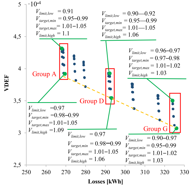
Fig. 11. VDEF-losses chart of the different simulations with only PV converters controlling voltage (CASE#1).
