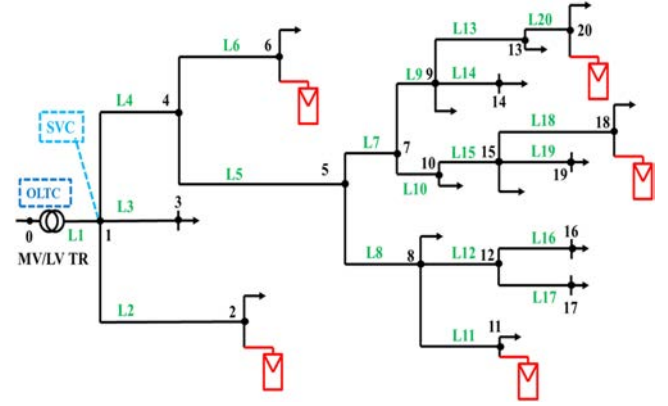
Fig. 7. LV grid under study corresponding to Case #1.
