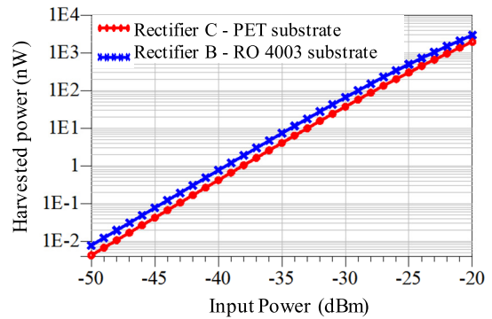
FIGURE 15. Simulated harvested power from rectifiers C using PET and rectifier B using RO 4003 substrate respectively, as function of input power with difference \Delta P between ports of 5 dB.
