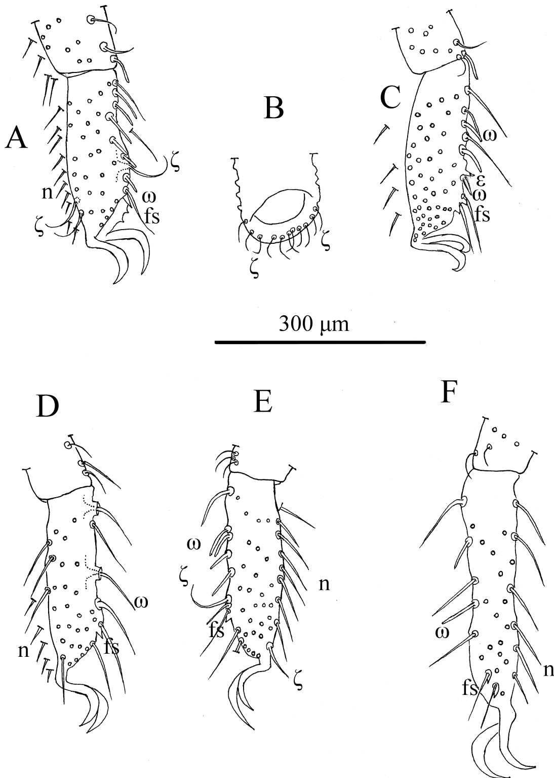
Figure 4 Paraplothrombium maketawa n. sp.: A – T-II anterior, n ventral spines; B – Ge-I distodorsal rim with fringe of \zeta at Ge-Ti joint; C – T-II posterior, \omega 0.6d semi-recumbent, non-clavate and \varepsilon ; D – T-III anterior; E – T-III posterior; F – T-IV posterior.
