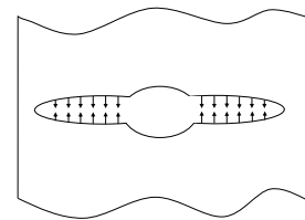
Fig. 2. The closure pressure in the crack wake
