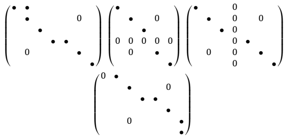
Fig. 6. Patterns for matrix m_t^p ; a • means \hat{f}_{p_i}(\bar{u}_j) > 0 .
