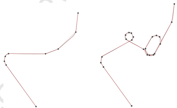
Fig. 3. Douglas–Peucker simplification of two sample trajectories (in red) with \epsilon = 1 km. The dashed lines connect the points selected by the algorithm. A trajectory put on holding stack yields more points than a regular approach. (For interpretation of the colours in the figure(s), the reader is referred to the web version of this article.)
