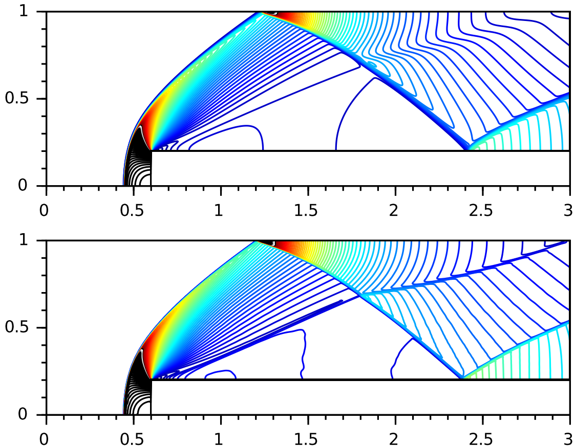
Figure 17: Simulation of the 2D Mach 3 wind tunnel with a step: Density with the first order scheme (up) and with the MUSCL/RK2 scheme (down)
