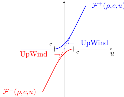
Figure 2: Comparison of the flux (2.5)–(2.6) and the UpWind flux for a fixed \rho .
