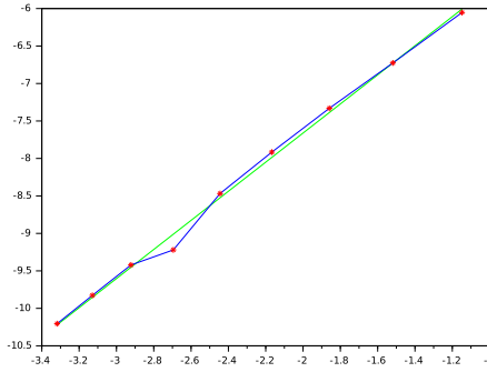
Figure 12: Maximal admissible time step \delta t as a function of 1 - \frac{\rho_m}{\rho^*} in blue; the green line has a slope 1.94.
